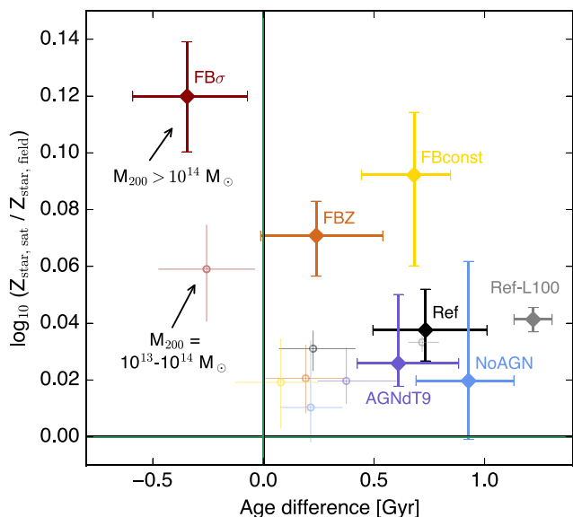
Figure 5. The difference between satellite and field galaxies in EAGLE ( 50 \text{ cMpc}^3 ) subgrid variation runs, in terms of mean stellar age ( x -axis) and stellar metallicity ( y -axis); shown are median values with statistical 1\sigma uncertainties indicated by error bars. Large diamonds with thick error bars represent satellites in (one) cluster of M_{200} \approx 10^{14} M_{\odot} , while small open circles and thin error bars denote the prediction for group haloes ( M_{200} = 10^{13}\text{--}10^{14} M_{\odot} ). For comparison, the two grey symbols show the corresponding values from the larger ( 100 \text{ cMpc}^3 ) Ref simulation discussed in the rest of this paper.
