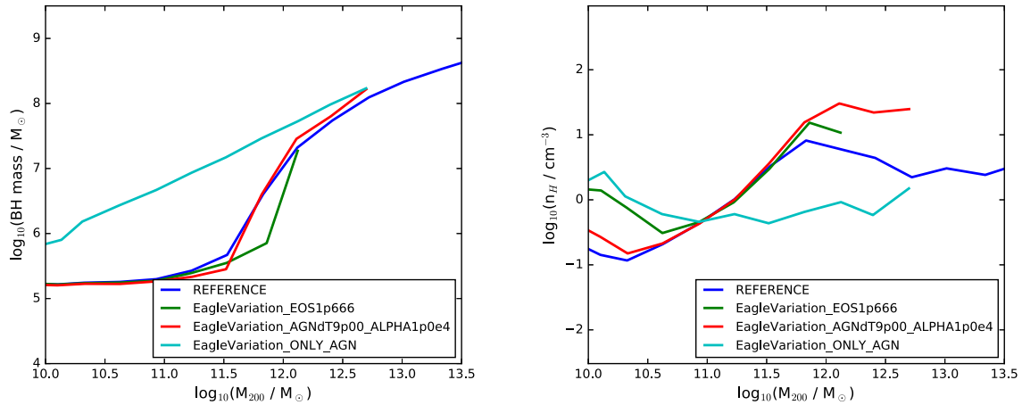
Figure 7. The panels in this figure are the same as in Fig. 6, but here we compare the reference simulation with simulations which vary the AGN feedback heating temperature and the ISM effective equation of state, as well as a model in which only AGN feedback is included (so that no star formation-driven outflow is present). The black hole mass–halo mass relations in the first two variations are remarkably similar, and the right-hand hand panel shows that densities around the black holes follow similar trends. This is expected since neither the detailed modelling of the ISM, nor the implementation of the AGN feedback, affect the halo gas adiabat which determines whether the star formation-driven outflow can regulate the central gas density. In contrast, the model in which energetic feedback from star formation is not implemented shows completely different behaviour. In particular, there is no break in the black hole mass–halo mass relation and black holes grow effectively in low-mass haloes so that their mass is limited by the halo binding energy rather than by the gas supply. This behaviour is predicted by the analytic model we have presented.
