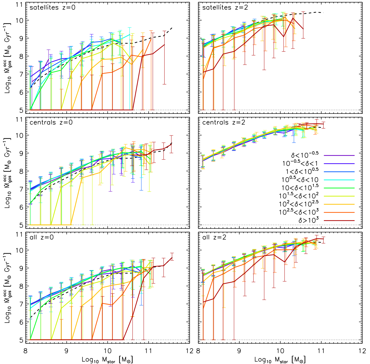
Figure 4. Median gas accretion rates as a function of stellar mass for satellites (top), centrals (middle) and all galaxies (bottom) at z=0 (left) and z=2 (right). Dotted and dashed curves are the same as in Fig. 2. Solid curves show median gas accretion rates in bins of galaxy overdensity, \delta \equiv \rho_{10}/\rho_{\text{all}} , as indicated in the legend. Gas accretion rates of zero have been set to 10^5 M_{\odot} \text{Gyr}^{-1} . Error bars show the 16th and 84th percentiles of the distribution. Only bins containing at least five galaxies are shown. There is a very strong dependence on galaxy overdensity at z=0 and a weaker dependence at z=2 . This dependence is primarily driven by satellite galaxies, although there is some residual dependence for centrals at z=0 .
