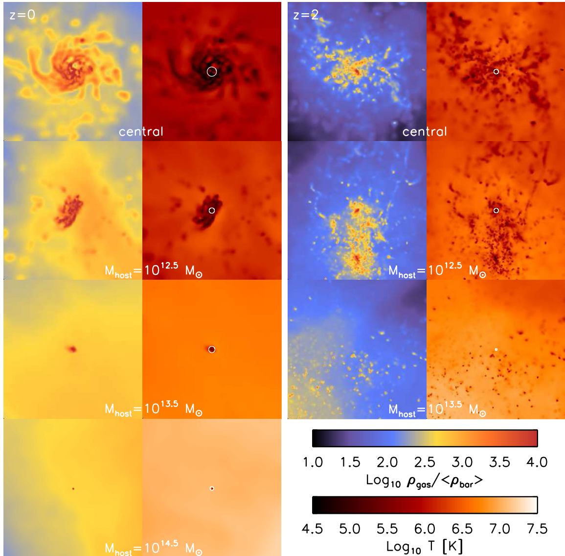
Figure 1. Projected ( 200 \text{ proper kpc})^3 images of the average gas overdensity (first and third columns) and temperature (second and fourth columns) at z = 0 (left) and z = 2 (right), each centred on a randomly chosen galaxy with M_{\text{star}} = 10^{10} M_{\odot} . White circles in the temperature panels indicate the galaxies’ stellar half-mass radii. The top row shows central galaxies, while the other rows show satellite galaxies for which the host halo mass increases from 10^{12.5} M_{\odot} (second row) to 10^{13.5} M_{\odot} (third row) to 10^{14.5} M_{\odot} (bottom row). The temperature of the surrounding gas increases with host halo mass, which increases the effect of the environment on gas accretion rates. At high redshift, there is much more cold, dense gas around the galaxies. Gas at the same overdensity also has a factor of 27 higher density at z = 2 than at z = 0 , because of the cosmological expansion of the Universe. Together, these effects result in a decrease of the environmental dependence with increasing redshift.
