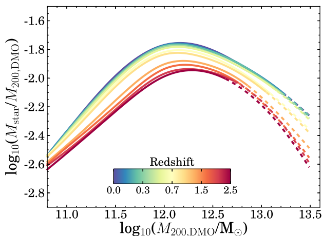
Figure 10. Evolution of the SMHM relation (left) and its scatter (right). Different from previous figures, we plot M_{\text{star}}/M_{200, \text{DMO}} along the y-axis in order to increase the dynamic range. Dashed lines indicate where there are fewer than 100 galaxies per halo mass bin of 0.4 dex width. With increasing redshift the normalization of the SMHMs drops and, except at the lowest halo masses, the scatter increases.
