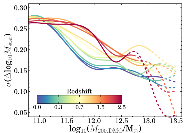
Figure 10. Evolution of the SMHM relation (left) and its scatter (right). Different from previous figures, we plot M_{\text{star}}/M_{200, \text{DMO}} along the y-axis in order to increase the dynamic range. Dashed lines indicate where there are fewer than 100 galaxies per halo mass bin of 0.4 dex width. With increasing redshift the normalization of the SMHMs drops and, except at the lowest halo masses, the scatter increases.
