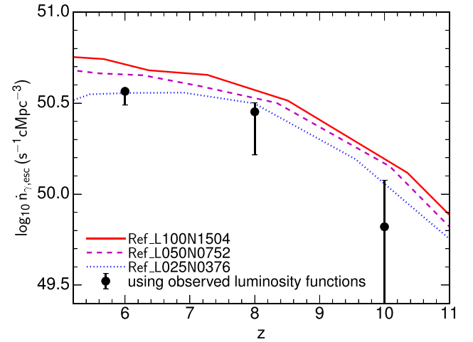
Figure 7. The rate at which ionizing photons escape from galaxies per unit comoving volume, \dot{n}_{\gamma,\text{esc}} , as a function of redshift using the EAGLE galaxy stellar mass function (dotted blue, dashed magenta and solid red curves correspond to simulations Ref-L025N0376, Ref-L050N0752 and Ref-L100N1504, respectively). Black symbols combine the observed 1500 Å luminosity function extrapolated to M_{1500,\text{AB}} = -13 from Bouwens et al. (2015a) with the evolution of the escape fraction taken from Fig. 5; error bars span the range covered if the faint-end slope is extrapolated to M_{1500,\text{AB}} = -10 and -16 .
