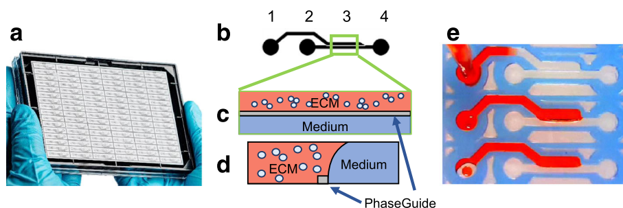
Fig. 1 Microtiter cancer-on-a-chip plate for 3D breast cancer therapy response testing. a Photo of OrganoPlate® platform consisting of 96 perfusable microfluidic chambers in parallel. b Closeup, (c) top and (d) side view of an individual chamber consisting of an ECM channel and a Medium channel. Cells are premixed into a gel solution, loaded into the ECM channel by capillary action and allowed to polymerize before the introduction of medium into the adjacent Medium channel for culture. PhaseGuide™ allows the gel solution to be pinned during the loading and polymerization step, thereby allowing support-free and unhindered exchange with the medium. e Photo demonstrates the filling of the ECM channel using a red dye
