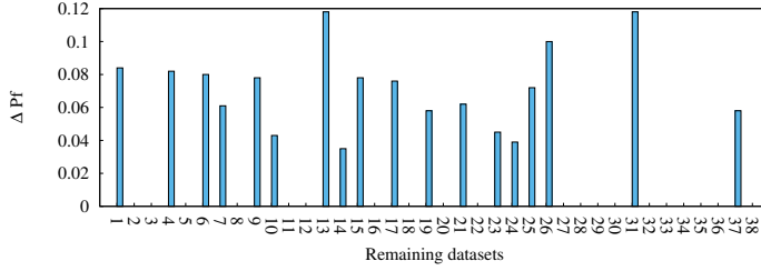
Fig. 5 Values of \Delta Pf of a potential competitor with respect to a_{best} on all datasets
