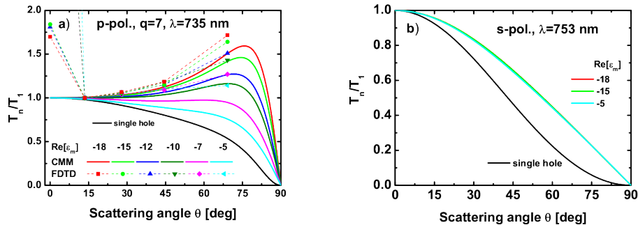
Fig. 4. Distribution of the transmitted power as a function of angle for different values of Re(\epsilon_m) , calculated with both CMM model and FDTD; for the latter we show T_n/T_1 , transmission per diffraction order normalized by the first diffraction order. Panel (a) is for p-polarization, while panel (b) renders the results for s-polarization.
