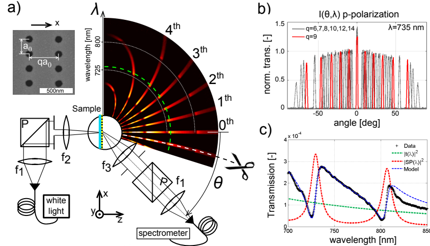
Fig. 1. (a) The goniometric setup used in the experiments. The sample is illuminated at normal incidence ( NA_{in} = 0.01 ) with a fiber-coupled white-light source. A second telescope ( NA_{out} = 0.03 ) scans, on a rotating stage, a semi-circle in the xz plane and collects the transmitted light at scattering angle \theta . Focal lengths are f_1 = 50 mm, f_2 = 75 mm, f_3 = 150 mm. Polarizers allow polarization-resolved study of the transmission. The false color plot reports the transmitted intensity I(\theta, \lambda) for the q = 9 array. The inset shows a detail of SEM image of sample with q = 2 . (b) Cross-cuts of I(\theta, \lambda) at fixed \lambda = 735 nm, i.e. along the green dashed arc indicated in a), for all the measured spacings q . (c) Transmission spectrum for the 1 st diffraction order of the 9a_0 array extracted along the white dashed line in a). The data are fitted with the model in Eq. (1). From the calculated parameters it is possible to separate the direct transmission |t|^2 (green dotted lines) and the resonant contribution |SP|^2 = |s/(u^{-1} - \sigma)|^2 (red dotted lines).
