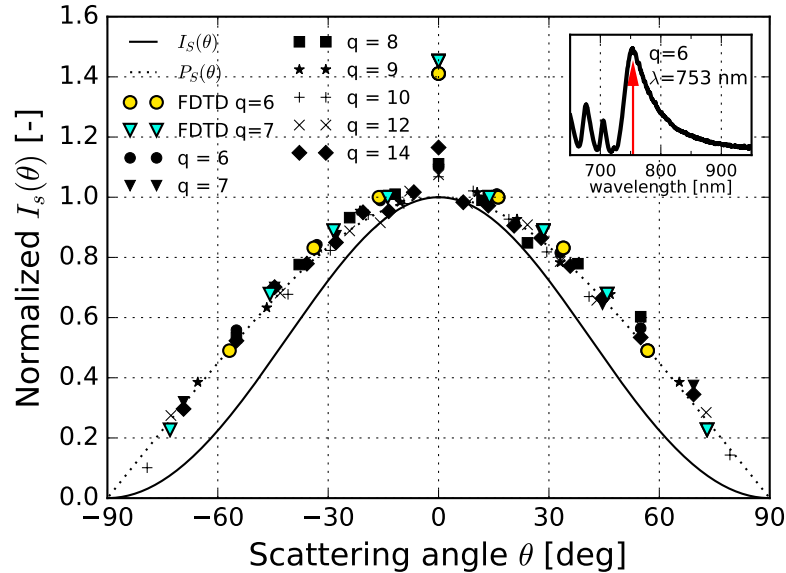
Fig. 3. Peak values for the resonance in the transmission spectra at different diffraction orders obtained with illumination with s-polarized light (peak position around 750 nm, shown in the inset) for detection on the air side. The solid curve shows the single-hole diffraction obtained with Eq. (3), while the dotted curve shows this result after correction by a factor \cos(\theta)^{-1} computed in Sec. 3 and discussed in Sec. 5. The latter curve overlaps with both the experimental data, as expected, and with the results of FDTD calculations of the power in each diffraction order, shown with yellow and cyan symbols.
