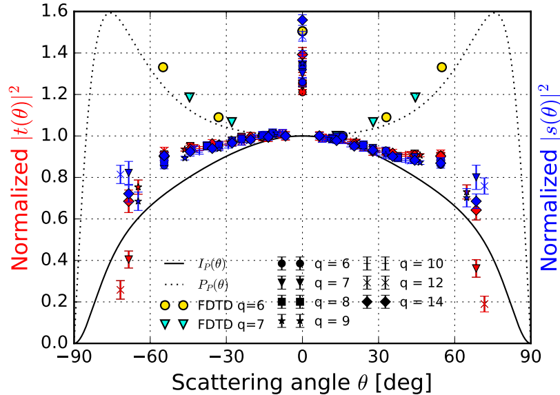
Fig. 2. Angular dependence of the parameters |t(\theta)|^2 (red symbols) and |s(\theta)|^2 (blue symbols), derived by fitting the model in Eq. (1) to the transmission diffraction orders measured for p-polarization on the air side of hole-arrays. Data from different arrays are normalized to the value for first orders; note the excellent consistency of parameters from arrays of different q -values. The excess intensity at \theta = 0 is due to incomplete absorption of light passing through the gold film. We report for comparison I_p(\theta) curve from Eq. (2) in solid line and, in dotted line, the curve including the correction with factor \cos(\theta)^{-1} computed in Sec. 3 and discussed in Sec. 5. The latter is in excellent agreement with FDTD calculations, shown with yellow and cyan symbols, for the power in each diffraction order.
