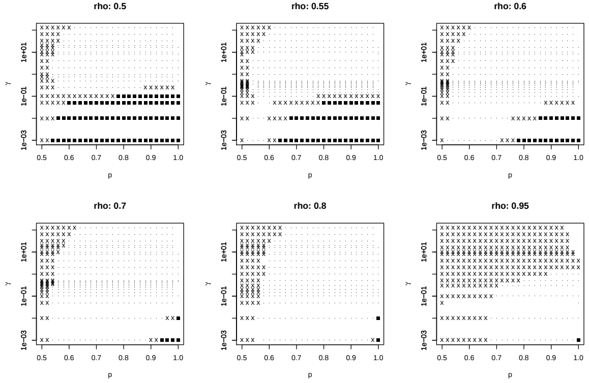
Figure 15: Sections of data supporting the phase diagram in Conjecture 3.5 increasing in \rho . Crosses, dots, and squares correspond to diffusive, super- and sub-diffusive regimes, respectively.
