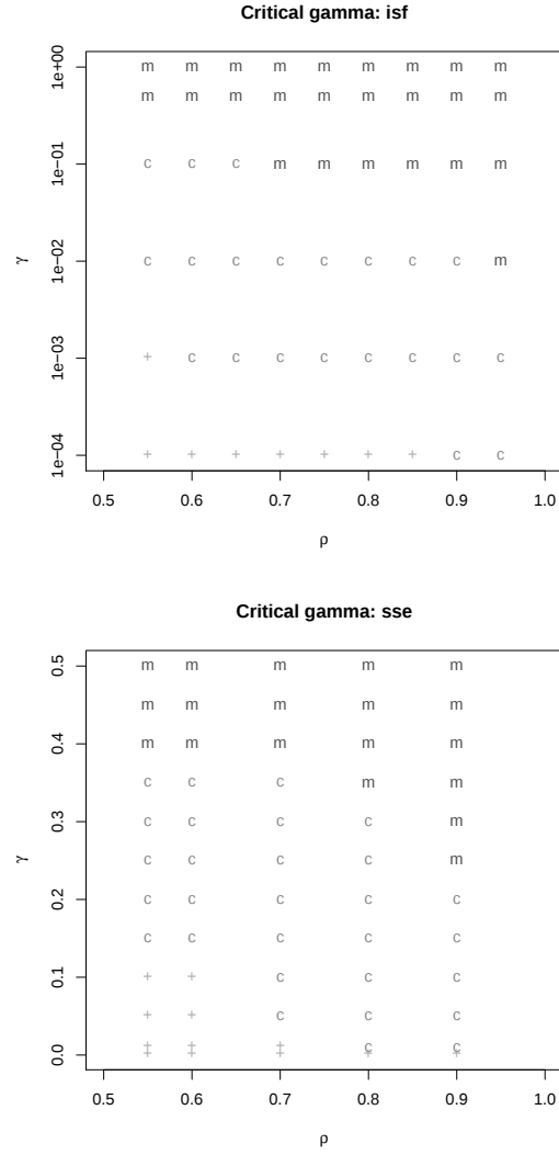
Figure 9: Quantitative phase diagrams describing Conjecture 3.4 in the ISF and the SSE environments. To each (\rho, \gamma) we associate the symbols m, c or +. They mean that the corresponding speed is a monotone, concave and non-concave function of p . \gamma_3(\rho) would correspond to the curve in between the regions of m's and c's, while \gamma_2(\rho) would be the line separating the regions with c's and +'s.
