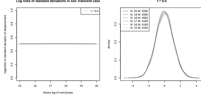
Figure 23: Transient, diffusive. (p, \rho, \gamma) = (0.56, 0.9, 0.001) . Estimated reliable time: \bar{n} = 2^{305} (see Section 4.2).
