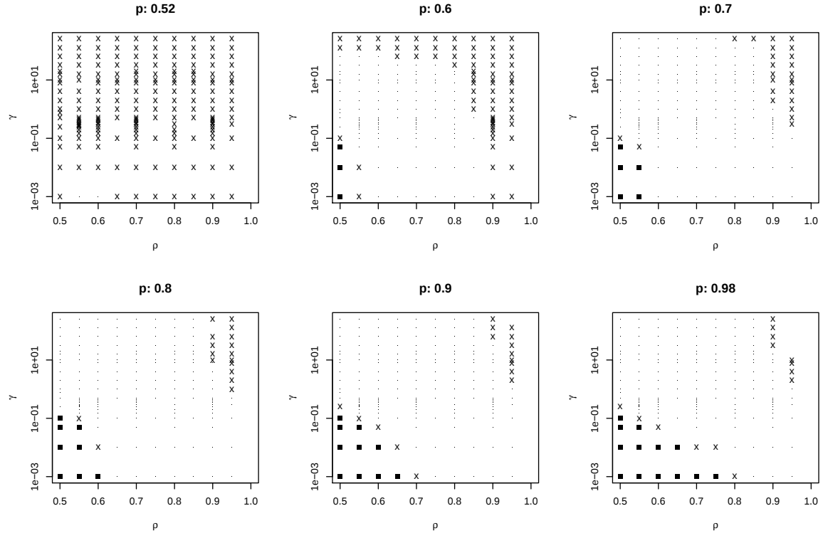
Figure 16: Sections of data supporting the phase diagram in Conjecture 3.5 increasing in p . Crosses, dots, and squares correspond to diffusive, super- and sub-diffusive regimes, respectively.
