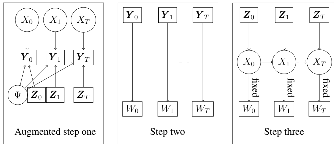
Figure 4. The steps of the augmented three-step LM model
