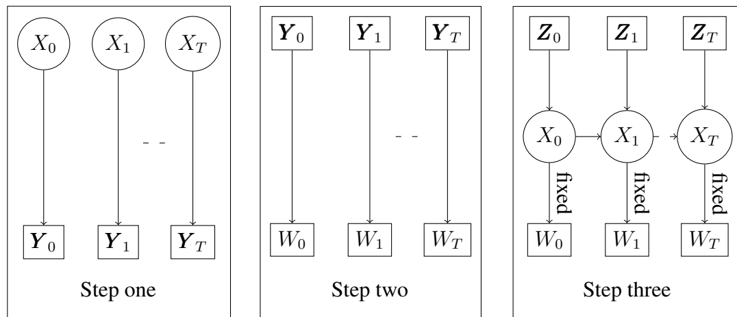
Figure 2. The steps of the three-step LM model
