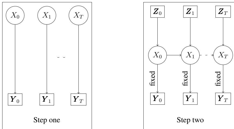
Figure 3. The steps of the two-step LM model
