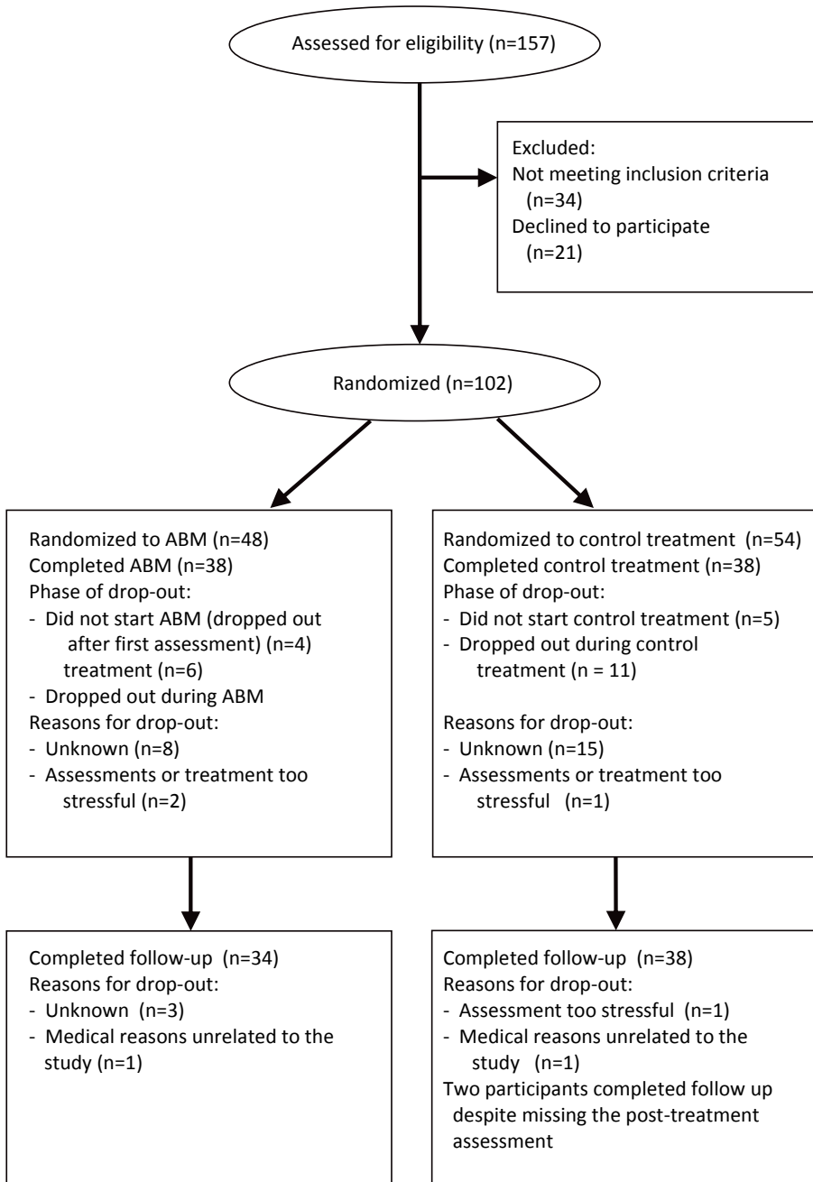
Figure 1. Flow chart
