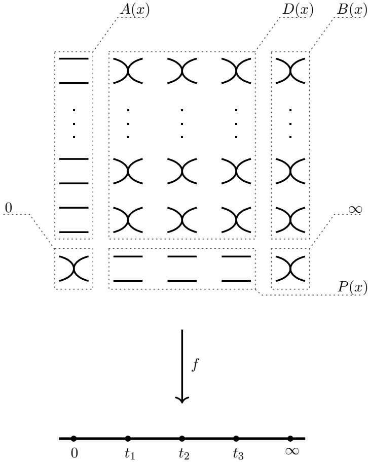
Figure 1.7: Ramification of f in the case of even degree.
