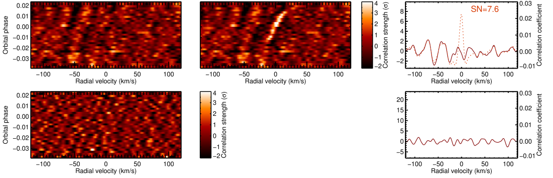
Figure 2.10: Top panels: Correlation coefficients for cross-correlation with the TiO template ( \text{VMR} = 10^{-7} ) between 640 nm and 670 nm, with and without injecting the template into the data prior to cross-correlation (middle and left panel, dashed and solid lines respectively). Restricting the wavelength range has reduced the signal-to-noise at which this template is retrieved after injection by over 9\sigma (compare to Figure 2.5), but it is not clear to what extent persistent inaccuracies still adversely affect the sensitivity of this restricted template. Bottom row: Correlation coefficients for cross-correlation with Barnard's star's optical spectrum. No enhanced correlation is observed. Given that the injection of the stellar absorption spectrum into the planetary transmission spectrum is not physically meaningful, the sensitivity of this non-detection can't straightforwardly be expressed in physical quantities like the limiting VMR.
