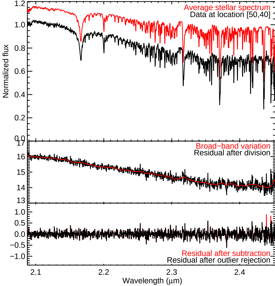
Figure 5.3: Stepwise removal of starlight from each spatial location in the data cubes.
