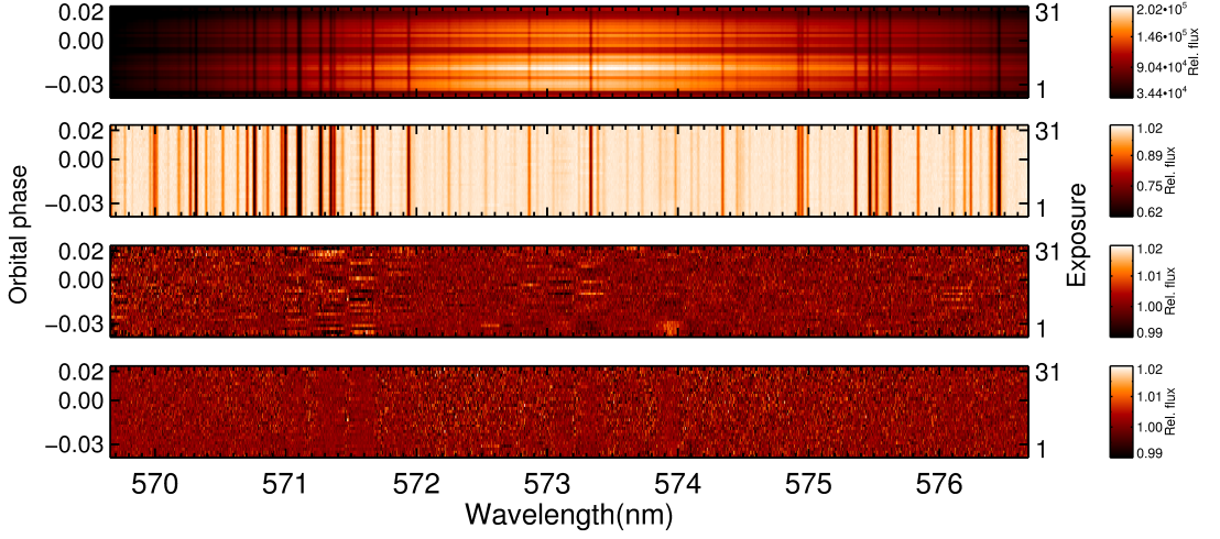
Figure 2.3: Major post processing steps of echelle order 17 before cross-correlation.
