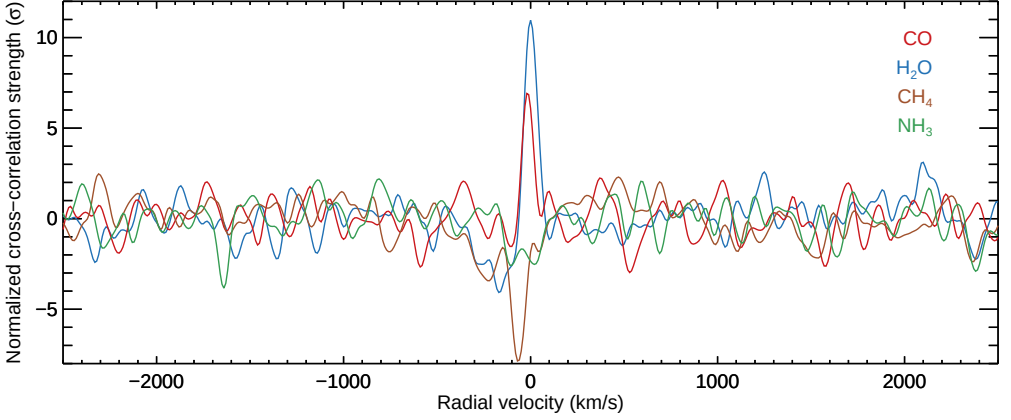
Figure 5.6: 1D cross-correlation functions of CO, H 2 O, CH 4 and NH 3 at the location of the planet normalized by their noise level.
