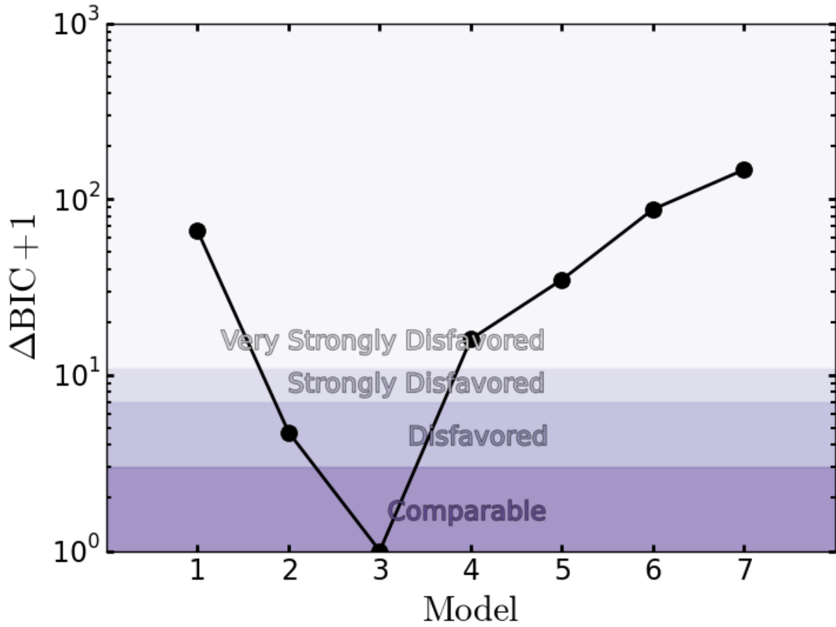
Fig. 8.— Plot of \Delta\text{BIC} (+1 due to the log axis) scores for the best fit 3D GMM models relative to the most preferred model. This most preferred model describes the system as a collection of three substructures, however, the two-substructure model is only disfavored and cannot be completely ruled out with certainty.
