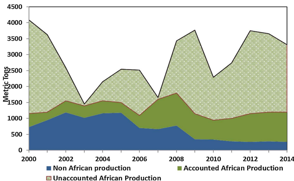
Fig. 8. Primary production versus unaccounted African production. Data on production include only tantalum ores and concentrates.
