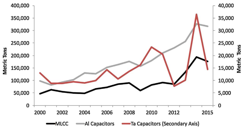
Fig. 13. Global trade in tantalum, multilayer ceramic, and aluminum capacitors.
