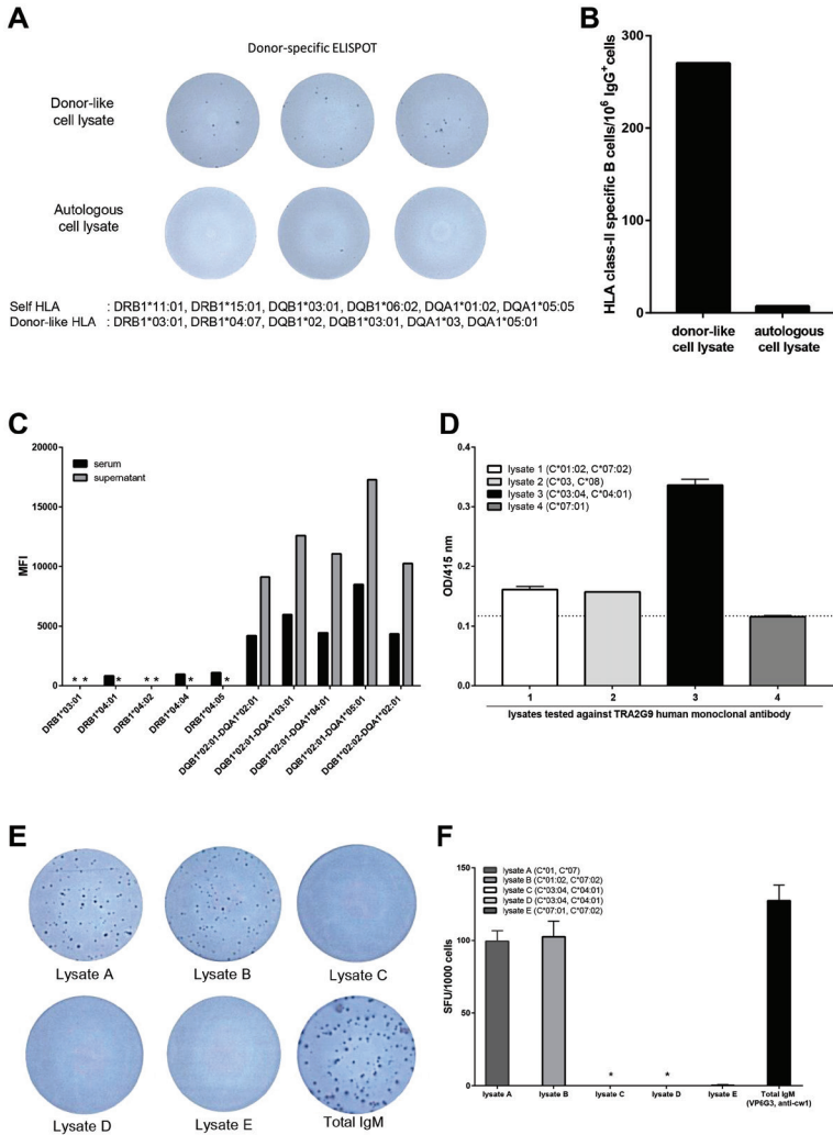
Supplementary figure 5: Detection of HLA-DQ and HLA-C antigens in lysate preparations. (A) HLA-DQ-specific memory B cells can be detected in the lysate-based ELISPOT assay. PBMC from a pregnancy-immunized woman (sample #201.1) was tested against a PBMC donor-like lysate (#13) lacking antibody positive HLA-DR specificities in order to detect solely HLA-DQ-specific memory B cells using the donor-specific memory B cell ELISPOT assay. (B) A frequency of 263 donor-specific memory B cells per million IgG producing cells were detected against the HLA class II present in the lysate whereas only background spots were observed against autologous lysate. (C) Isolated HLA-DQ2 directed antibodies were detected in serum and culture supernatants harvested upon 6-day polyclonal activation by Luminex single antigen bead assays, confirming that spots detected were specific for HLA-DQ. (D) HLA-C molecules are present in lysate preparations. Lysates containing different HLA-C antigens were coated onto ELISA plates by anti-beta-2 microglobulin coating antibody and then tested against a human monoclonal antibody (TRA2G9) recognizing HLA-C*01:02, C*03:02, C*03:03, C*03:04, C*04:01, C*14:01. Reactivity of the monoclonal antibody with corresponding HLA-C antigens in lysates 1, 2 and 3 could be detected using a goat-anti-human IgM antibody. OD: optic density. (E) HLA-C molecules can be detected in ELISPOT format. The HLA-Cw1-specific IgM producing hybridoma VP6G3 was tested against lysates containing various HLA-C molecules (lysate A: C*01, C*07, lysate B: C*01:02, C*07:02, lysate C: C*03:04, C*04:01, lysate D: C*03:04, C*04:01 and lysate E: C*07:01, C*07:02). Only lysates containing HLA-C*01 gave rise to spot formation. (F) Quantification of HLA-C specific ELISPOT assay.
