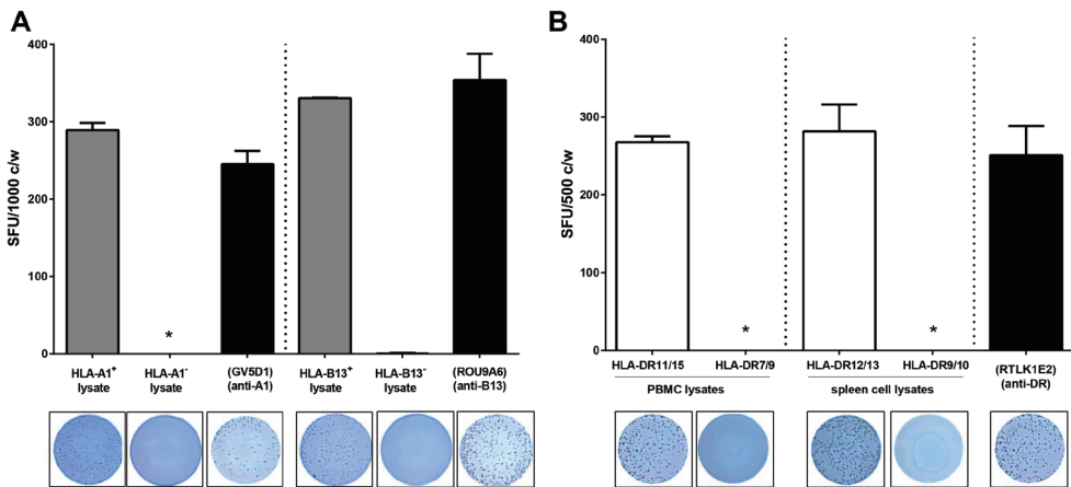
Figure 3. Lysates prepared from peripheral blood mononuclear cells (PBMCs) or spleen cells can be used to detect HLA antibody-producing cells with correct specificity. (A) A PBMC lysate containing HLA-A1 or HLA-B13 only gave spot formation with only an HLA-A1 or HLA-B13 specific antibody-producing hybridoma, whereas no spot formation was observed with a PBMC lysate lacking either HLA-A1 or HLA-B13 (gray bars). (B) Spot formation was observed only when an HLA-DR3, -DR8, -DR11, -DR12, -DR13 or DR14-specific hybridoma was tested against PBMC or spleen cell lysates containing HLA-DR11 and -DR15, or HLA-DR12 and -DR13 (white bars) and not against lysates containing HLA-DR7 and -DR9, or HLA-DR9 and -DR10. In all cases, number of spots detected by donor-specific ELISPOT assays were comparable to those detected by total IgG ELISPOT assays (black bars). (*): No SFU detected. Error bars represent the mean \pm SD of triplicate wells. Results are representative of experiments performed with four different lysates. SFU: spot forming units.
