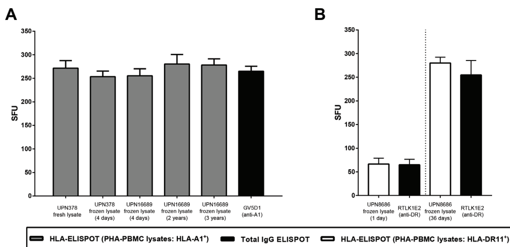
Figure 2. HLA in lysates remain stable upon freezing-thawing. (A) Comparable numbers of spots were obtained when HLA-A1 + lysates prepared from PHA stimulated PBMC samples were used immediately after preparation (fresh) or frozen for 4 days up to 3 years (gray bars) and then used to detect HLA-A1 antibody-producing cells (GV5D1, black bar). (B) Similarly, all HLA-DR11 antibody-producing cells were detected at high sensitivity similar to total IgG ELISPOT assay (RTLK1E2, black bars) when HLA-DR11 + cell lysates (white bars) frozen for short (1 day) or longer term (36 days) were used. Error bars represent the mean \pm SD of triplicate wells. Results are representative of experiments performed with four different lysates. ELISPOT, enzyme-linked immunospot; PBMC, peripheral blood mononuclear cell; PHA, phytohemagglutinin; SFU, spot forming units.
