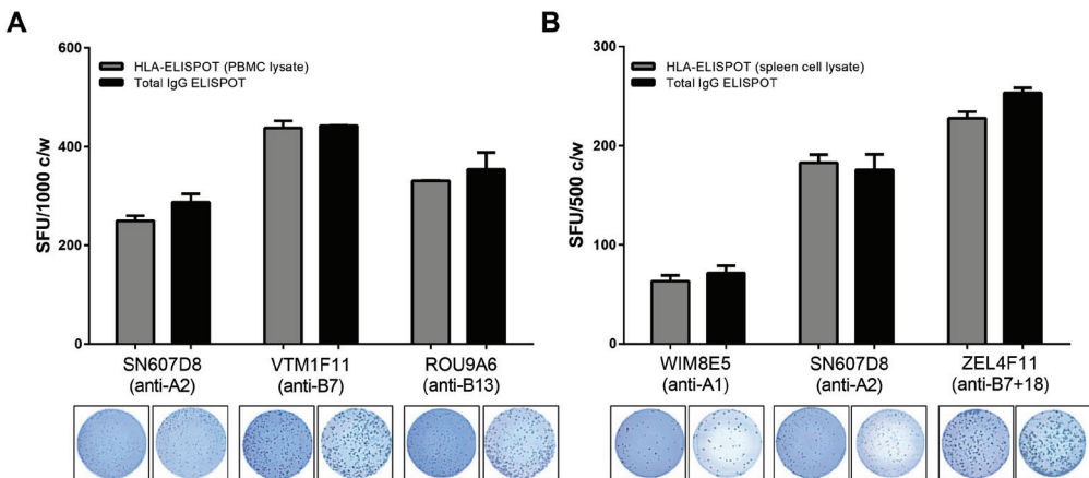
Figure 1. Lysates can be used to detect HLA-antibody producing cells with high sensitivity. (A) One PBMC lysate (positive for HLA-A2, HLA-B7 and HLA-B13) was tested against three different hybridomas producing HLA antibodies of the corresponding specificity. Comparable numbers of spots were found for each HLA in the lysate using donor-specific enzyme-linked immunospot (ELISPOT; gray bars) and concurrent total IgG ELISPOT assays (black bars). (B) All antibody-producing cells were detected using spleen cell lysates (positive for HLA-A1, HLA-A2, HLA-B7 and HLA-B18). Error bars represent the mean \pm SD of triplicate wells. Results are representative of experiments performed with four different lysates. SFU, spot forming units.
