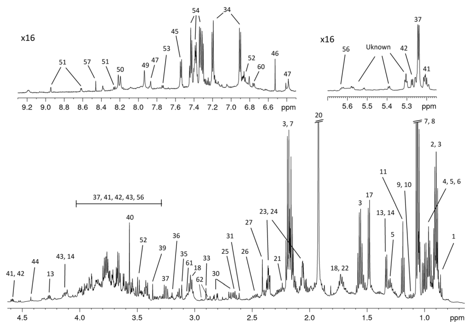
Fig. 2 Regions of the 600 MHz ^1\text{H} NMR spectrum of the pool sample mix of all fecal extracts used in this study. The regions on top are multiplied 16 times for better visualization. 60 fecal metabolites were identified with most of them annotated on the spectrum. Metabolites and their numbering as displayed in figure: 1: 2-methylbutyrate; 2: Valerate; 3: n-butyrate; 4: Leucine; 5: Isoleucine; 6: Valine; 7: Propionate; 8: Isobutyrate; 9: 3-methyl-2-oxoisovalerate; 10: 2-oxoisovalerate; 11: Ethanol; 12: 3-hydroxybutyrate; 13: Threonine; 14: Lactate; 15: 2-hydroxyisobutyrate; 16: 3-hydroxy-2-butanone; 17: Alanine; 18: Lysine; 19: Thymine; 20: Acetate; 21: 5-aminopentanoate; 22: Ornithine; 23: Proline; 24: Glutamate; 25: Methionine; 26: Glutamine; 27: Succinate; 28: 2-oxoglutarate; 29: 3-phenylpropionate; 30: Aspartate; 31: Methylamine; 32: Malate; 33: Trimethylamine; 34: Tyrosine; 35: Malonate; 36: Choline; 37: D-glucose; 38: Taurine; 39: Methanol; 40: Glycine; 41: D-xylose; 42: D-galactose; 43: Fructose; 44: Dihydroxyacetone; 45: Uracil; 46: Fumarate; 47: Urocanate; 48: Ethanolamine; 49: Xanthine; 50: Hypoxanthine; 51: Nicotinate; 52: 3-hydroxyphenylacetate; 53: Tryptophan; 54: Phenylalanine; 55: Orotate; 56: UDP-glucuronate; 57: Formate; 58: Benzoate; 59: 4-aminohippurate; 60: Homovanillate; 61: Putrescine; 62: Asparagine
