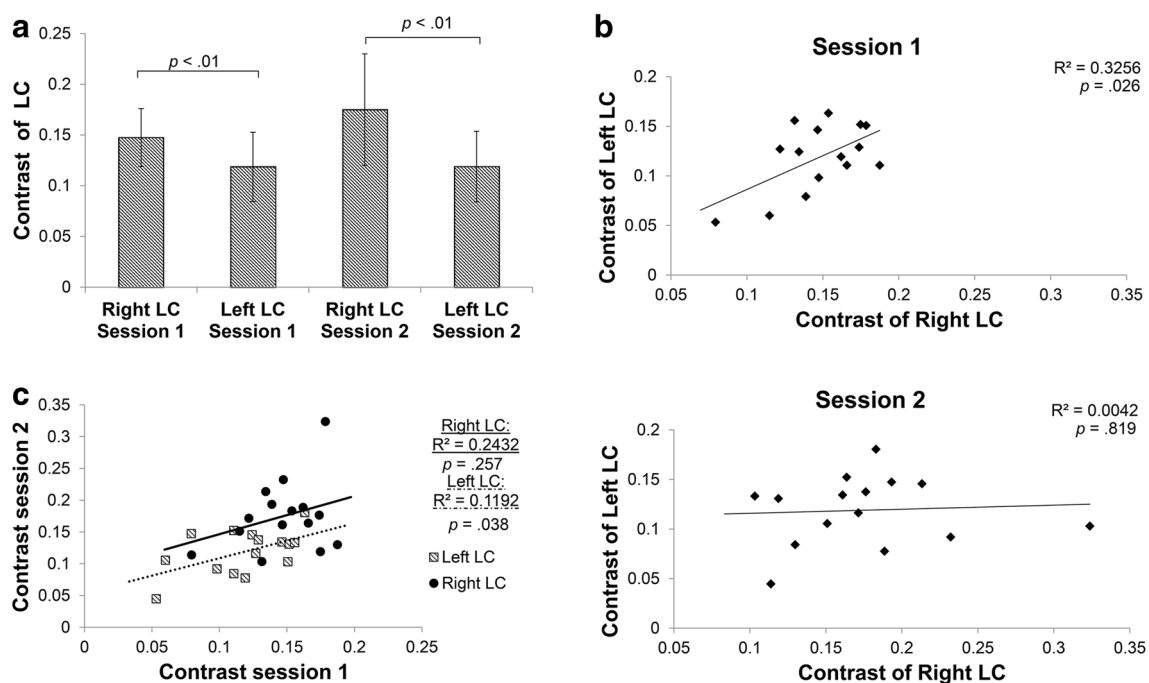
Fig. 4 ROI analysis examining the test–retest reliability of the MRI contrast. a Contrast of the right and left LC for the first (left) and second scan session (right). Bars indicate mean \pm standard deviation.
