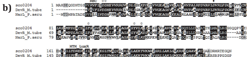
FIGURE S1: Alignment of SCO0203 (OsdK) and SCO0204 (OsdR).
