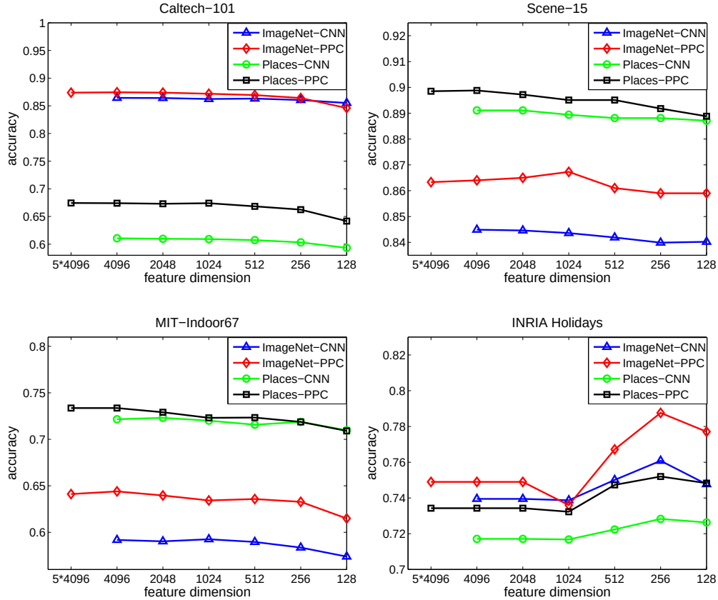
Figure 3.4: Comparisons of CNN and PPC on different dimensions
