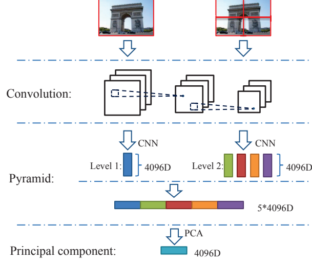
Figure 3.1: The procedure of PPC algorithm.
