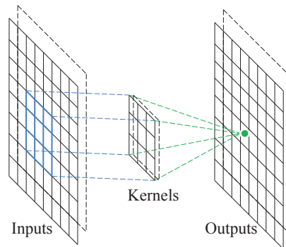
Figure 2.3: The operation of the convolutional layer.
