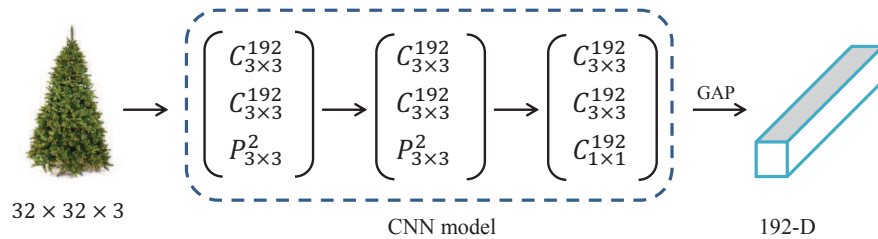
Figure 5.5: The CNN baseline proposed in [263].
