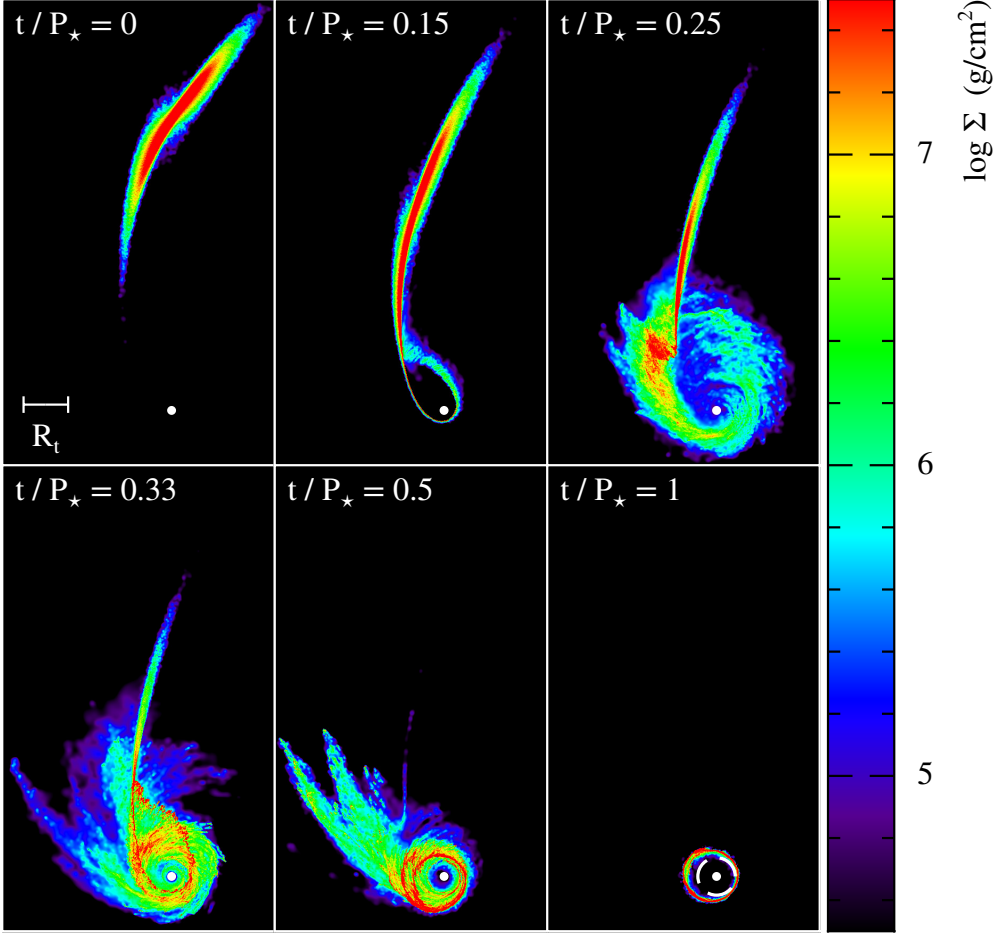
Figure 2.12: Snapshots of the fallback of the debris at different times t/P_* = 0, 0.15, 0.5 and 1 for models RI5e.95. For this model, the period of the star P_* is 22 h. The colours correspond to the column density \Sigma of the gas whose value is indicated on the colour bar. The white point represents the black hole. The dashed white circle on the last snapshot represents the circularization radius given by equation (2.13) for the relativistic potential. The stream is longer for this model than for model RI5e.8 as the eccentricity is larger. As a result, the self-crossings involve a larger fraction of the debris, causing them to move faster to circular orbits.
