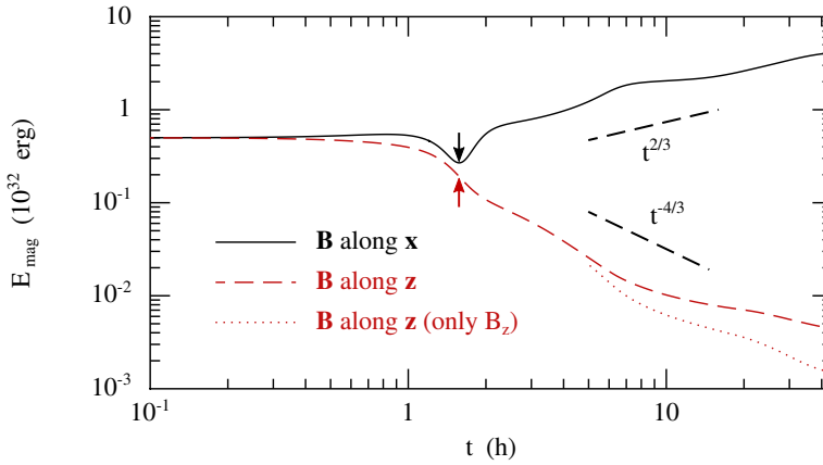
Figure 5.3: Magnetic energy evolution for models F1B1G-x (black solid line) and F1B1G-z (red dashed line), for which the penetration factor is \beta = 1 . The dotted red line shows the magnetic energy computed from the z component of the field only for model F1B1G-z. The times of pericentre passage are indicated by the arrows on each curve. The two solid dashed segments indicate the scalings that the magnetic energy is expected to follow after the disruption.
