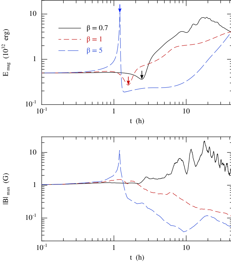
Figure 5.4: Magnetic energy (upper panel) and maximal magnetic field strength (lower panel) evolution for models P.7B1G-x (black solid line), F1B1G-x (red dashed line) and F5B1G-x (long-dashed blue line). The times of pericentre passage are indicated by the arrows on each curve.
