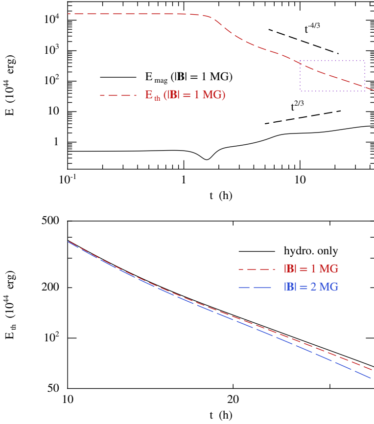
Figure 5.8: Evolution of the magnetic (black solid line) and thermal (red dashed line) energies for model F1B1MG-x (upper panel). The dashed black segments indicate the scaling that these energies are expected to follow after the disruption. The area delimited by the dotted purple rectangle is zoomed-in on the lower panel, which shows the late time thermal energy evolution for models F1B0G (solid black line), F1B1MG-x (dashed red line) and F1B2MG-x (long-dashed blue line).
