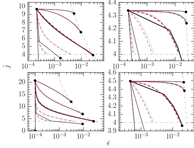
Figure 3.5: Stream evolution shown in the \bar{j} - \bar{\epsilon} plane for various values of the parameters. The meaning of the different lines are the same as in Fig. 3.3. In each panel, the five sets of curves correspond to different values of the magnetic efficiency v_A/v_c = 0.01, 0.03, 0.1, 0.3 and 1 (from top to bottom). The different panels correspond to different values of M_h and \beta . The two top panels show M_h = 10^6 M_\odot for \beta = 1 (upper left) and for \beta = 5 (upper right). The two bottom panels adopt \beta = 1 for M_h = 10^5 M_\odot (lower left) and M_h = 10^7 M_\odot (lower right). The set of thicker curves is associated to a magnetic stresses efficiency v_A/v_c = 0.1 , which approximately corresponds to the critical value (equation (3.20)) defining the boundary between circularization and ballistic accretion, independently on M_h and \beta .
