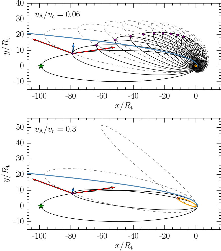
Figure 3.2: Stream evolution for two magnetic stresses efficiencies v_A/v_c = 0.06 (upper panel) and 0.3 (lower panel). The black hole mass and penetration factor are fixed to M_h = 10^6 M_\odot and \beta = 1 . The black hole is at the origin. The succession of ellipses starts from the orbit of the most bound debris, whose apocentre is indicated by a green star on the left of the figure. Each stream orbit is divided into two ellipses. The stream elements moving towards the black hole follow the black ellipses. The dashed grey ellipses, precessed with respect to the black ones, are covered by the gas elements moving away from the black hole after pericentre passage. The intersection point is located where the black and grey ellipses cross. At this point, the orbit of the stream changes due to shocks and magnetic stresses. The stream elements then infall towards the black hole on the next solid black ellipse. The first ten self-crossing points are indicated by the purple dots. At the first crossing point, where the transition between orbit 0 and 1 happens, the red arrows show the velocity of the components involved in the associated shock, \mathbf{v}_0^{\text{in}} and \mathbf{v}_0^{\text{out}} . The blue arrow indicates the initial velocity of orbit 1, \mathbf{v}_1 , after the debris experienced both shocks and magnetic stresses. This situation is also illustrated in Fig. 3.1 for N = 0 . The final orbit of the stream, for which one of the two stopping criteria is satisfied, is depicted in orange. For v_A/v_c = 0.06 , the stream circularizes to form a disc. For v_A/v_c = 0.3 , the stream is ballistically accreted before circularizing. The blue line represents a parabolic trajectory with pericentre R_p , equal to that of the star. The trajectories of the debris falling back towards the black hole within the tail are therefore contained between this line and the orbit of the most bound debris.
