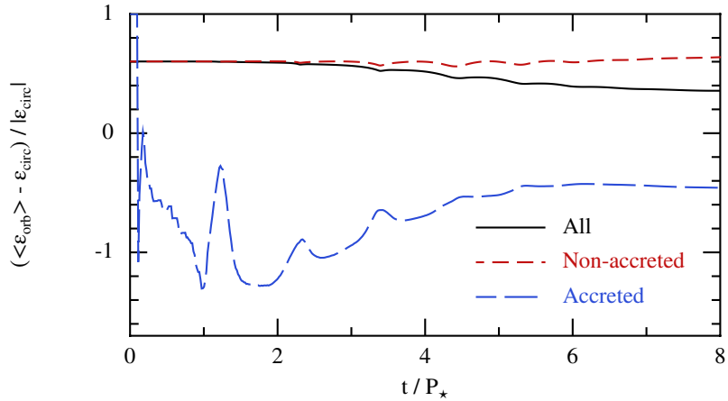
Figure 2.7: Evolution of the average specific orbital energy of all the debris, the non-accreted and accreted ones for model RA5e.8. For this model, the period of the star P_{\star} is 2.8 h. The average specific orbital energy is shown relative to the specific circularization energy given by equation (2.15) for the relativistic potential.
