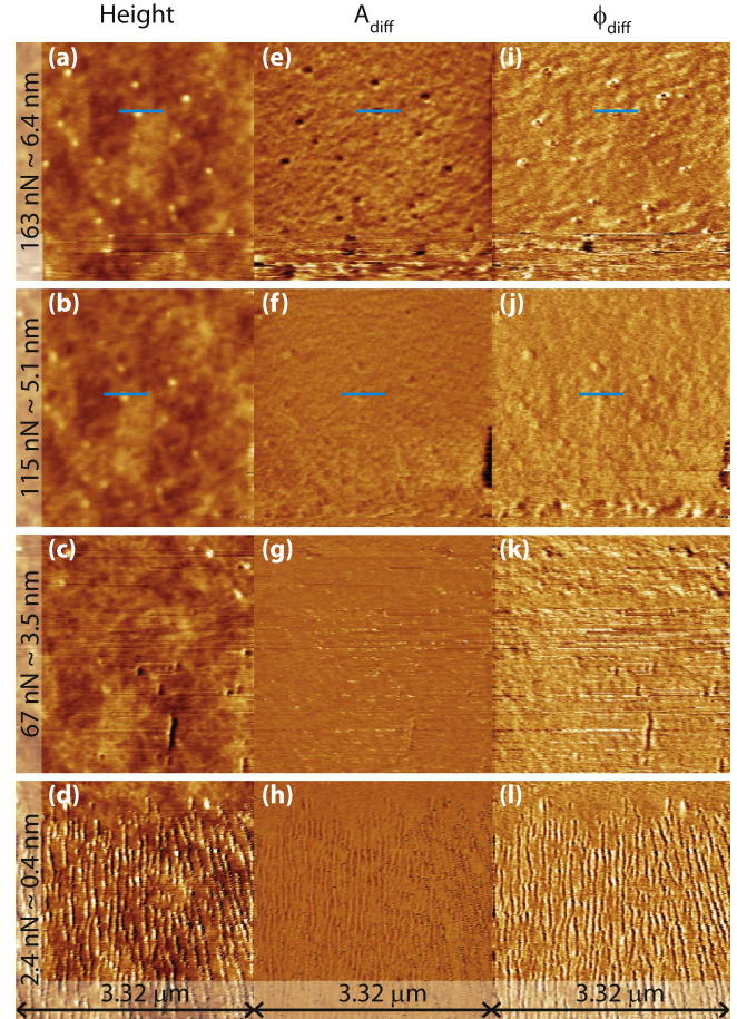
Figure 3. HFM measurements for different contact forces: from left to right measured simultaneously: the height (a)–(d) and both the amplitude A_{\text{diff}} (e)–(h) and the phase \phi_{\text{diff}} (i)–(l) of the difference frequency. The contact force F_c as well as the resulting average indentation into the sample are indicated at the left in the height images. The gold nanoparticles are only visible at a contact force of 163 and 115 nN. At these forces, they are not only visible in A_{\text{diff}} and \phi_{\text{diff}} , but also in the height image. We ‘loose’ the nanoparticles in the height, A_{\text{diff}} , and \phi_{\text{diff}} with decreasing force. At a F_c = 2.4 nN, we observe that we damaged the surface, while measuring at higher forces. All height, A_{\text{diff}} , or \phi_{\text{diff}} images have the same (color) range such that the contrast for different contact forces can be compared directly. We provide typical cross sections with absolute values of the height, A_{\text{diff}} , and \phi_{\text{diff}} at the positions of the nanoparticles in figure 4.
