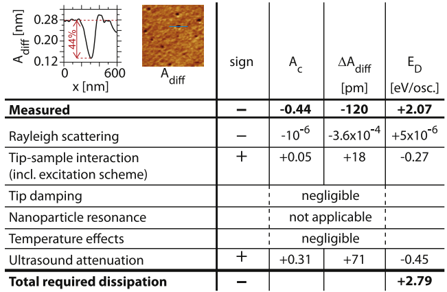
Figure 6. Experimentally determined dissipation based on friction at the nanoparticle-polymer interface: we measure holes in A_{\text{diff}} that require a dissipation of 2.07 \text{ eV osc.}^{-1} . To provide an overview, we list also the contribution of all other contrast mechanisms that (partly) take place simultaneously. The measured dissipation must be slightly higher than determined ( 2.79 \text{ eV osc.}^{-1} instead of 2.07 \text{ eV osc.}^{-1} ), as both tip-sample interaction and ultrasound attenuation are not negligible and have, in addition, an inverted sign in the contrast.
