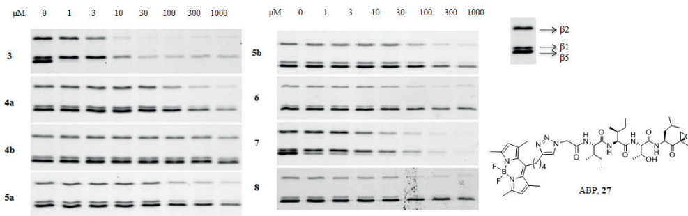
Figure 4. Inhibition profile of compounds 3-8 and the structure of ABP ( 27 ).
