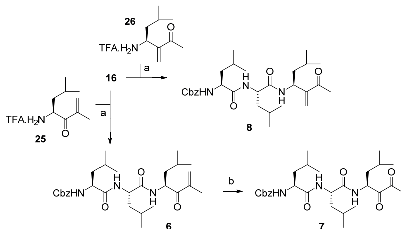
Scheme 3. Synthesis of 6 and 7 .
