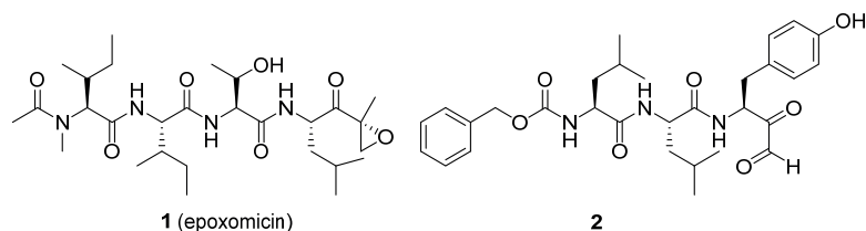
Figure 1. Structures of epoxomicin (1) and peptide \alpha -keto-aldehyde (2) that are at the basis of the here presented studies.
