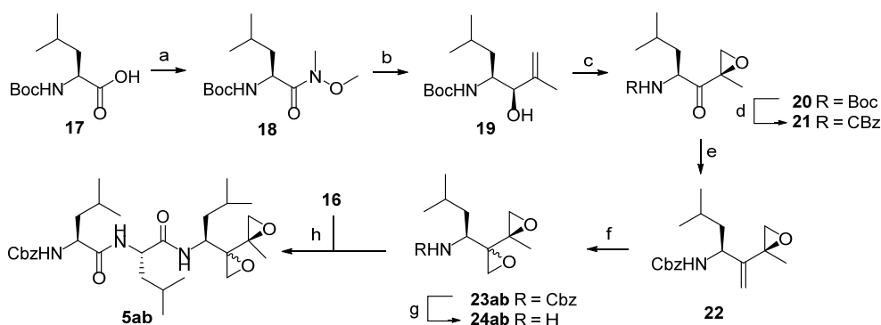
Scheme 2. Synthesis of compounds 5a and 5b .
