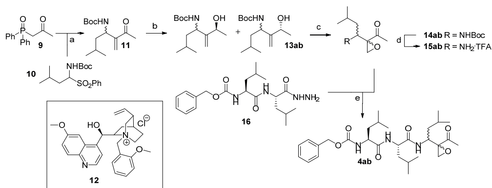
Scheme 1. Synthesis of 4ab .
