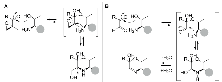
Figure 2. Mechanism of peptide epoxyketone (A) and peptide \alpha -keto-aldehyde (B) mediated proteasome inactivation.
