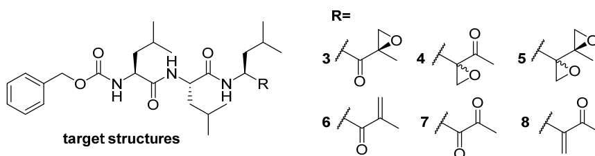
Figure 3. Target structures 3-8 that are at the basis of the here-presented studies
