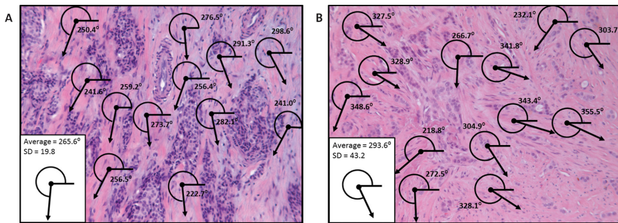
Figure 1. (A) example of breast tumor biopsy with linearly aligned stroma. (B) example of breast tumor biopsy with disorganised stroma.
