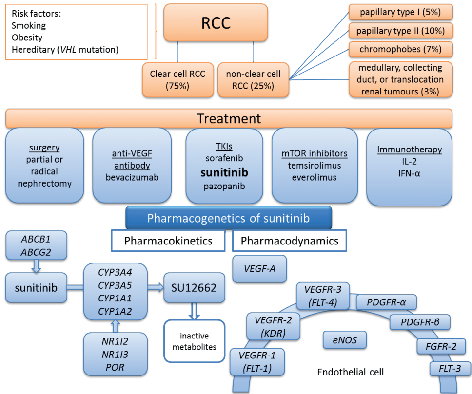
Figure 1: Overview of RCC risk factors, tumor types, and treatment options with a focus on sunitinib and pharmacogenetics of sunitinib in mRCC.
