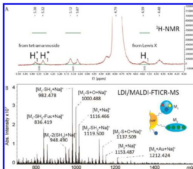
Figure 6. (A) ^1H NMR spectrum of AuNPs functionalized with both Lewis X and tetramannoside ligands in D_2O at 500 MHz. A detailed description of the NMR spectrum is reported in Supporting Information Figure S13. (B) LDI/MALDI-FTICR MS spectrum of AuNPs functionalized with both Lewis X and tetramannoside ligands.
