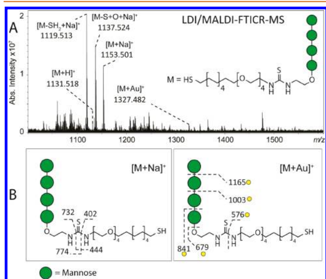
Figure 5. (A) LDI/MALDI-FTICR MS spectrum of AuNP functionalized with tetramannoside-based ligand. The tetramannoside-based ligand was detected as [M + H]^+ , and [M + Au]^+ at low intensity, and detected as [M + Na]^+ , [M-SH_2 + Na]^+ and [M-S + O + Na]^+ at higher intensities. (B) Structure characterization performed by CID confirmed the identity of these species. Fragmentation of [M + Au]^+ allowed characterization of the carbohydrate moiety of the ligand, whereas CID analysis of [M + Na]^+ provided more information on the structure of the linker. Yellow circles indicate gold-linked fragment ions.
