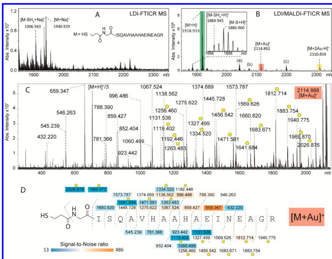
Figure 2. Relevant parts of the FTICR mass spectra of AuNPs with OVA 323-339 peptide-based ligand obtained from LDI only (A) and LDI/MALDI (B). The use of 1,5-DAN as a MALDI matrix resulted in the detection of pseudomolecular ions [M + H]^+ , [M + Au]^+ , and [M + 2Au - H]^+ , highlighted with three different colors. Additional pseudomolecular ions observed were (a) [M - S - H + 1,5\text{-DAN}]^+ at m/z 2043.030, (b) [M - H + 1,5\text{-DAN}]^+ at m/z 2074.998, and (c) pseudomolecular ion of coupled glucose-based and OVA-based ligands at m/z 2199.038 (as explained in the Results and Discussion section). Further structure characterization of [M + Au]^+ , [M + H]^+ , and [M + 2Au - H]^+ was performed by collision-induced dissociation (CID) and as an example the tandem mass spectrum of the first species is shown in C (the other two can be found in Figure S2). The obtained high sequence coverages (D) allowed to determine the preferred coordination site(s) of Au^+ by evaluating all gold-containing fragment ions (indicated with yellow circles).
