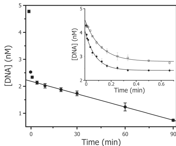
Figure 3. Solution kinetics of DNA cleavage by SfiI. The reactions contained 5 nM [ ^3H ] pGB1 \Delta 466 and 3 nM WT SfiI in Mg^{2+} buffer at 21.5^{\circ}C . Displayed is the remaining SC DNA left as a function of time. In the main panel, the linear regime between t = 5 and t = 90 min is fitted to a straight line. The inset shows the pre-steady state kinetics obtained with the rapid quench-flow device: either by pre-mixing WT SfiI with the DNA before initiating the reaction with MgCl_2 (black circles); or by adding the DNA to a solution containing the protein and the MgCl_2 (open squares). The results are exponentially distributed with decay constants of, respectively, 2.5 \times 10^{-1} s^{-1} and 1.2 \times 10^{-1} s^{-1} (black lines).
