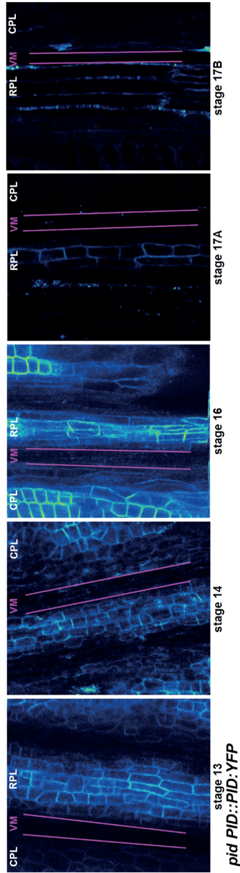
Figure S4: PID is repressed in the valve margin.
