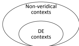
Figure 1: The subset relationship between DE and non-veridical contexts
