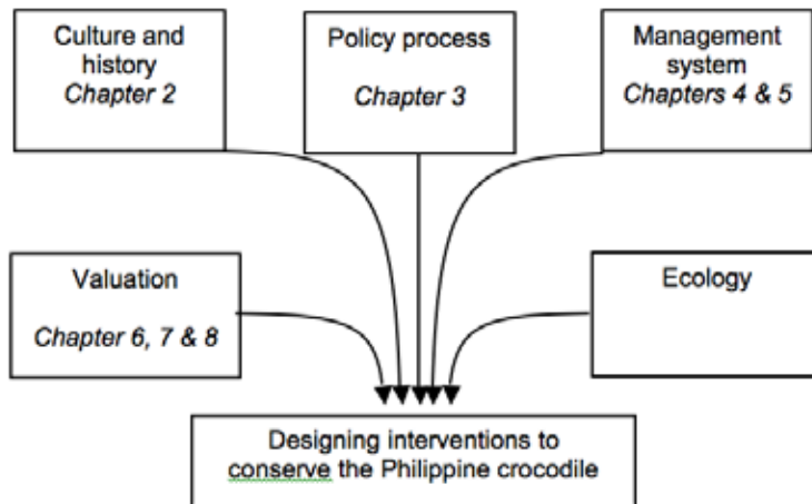
Figure 1.2: Schematic representation of key dimensions necessary for analyzing and crafting solutions for complex conservation problems (Clark et al. 1996: 943). The corresponding chapters in this thesis are indicated in italics.
