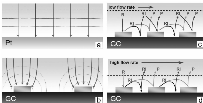
Figure 2.6: Mass transport towards electrodes: diffusion towards an infinite planar electrode is linear (a), while well-separated NPs show radial diffusion spheres (b). As the inter-NP distance is decreased, the diffusion spheres start to overlap. In (c) and (d), the influence of flow rate on mass transport to a NP array is illustrated: at low flow-rate, the diffusion layer is large and there is a chance for reaction intermediates (RI) generated at a NP to re-adsorb on adjacent NPs (c). When the flow-rate is increased, the diffusion layer effectively becomes thinner and RIs are less likely to re-adsorb, escaping from the NP ensemble (d). Adapted from ref [208]. ©2010, The Electrochemical Society.
