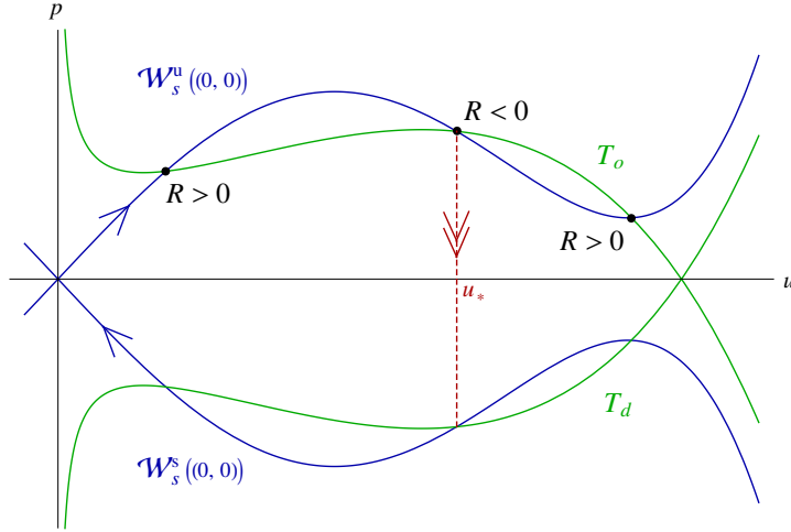
Figure 3.8: The coefficient R (3.94) interpreted geometrically as the relative slope of T_o with respect to W_s^u((0,0)) at their intersection point. Only the homoclinic pulse associated to the second intersection can be stable (Lemma 3.34).
