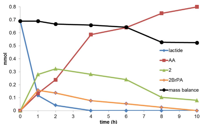
Figure 1. Rearrangement of lactide to acrylic acid at 175 °C as a function of time. Reaction conditions: lactide (0.69 mmol), HOMs (0.83 equiv), PPh 4 Br (5 equiv), sulfolane. Lines are only given as a guide to the eye.
