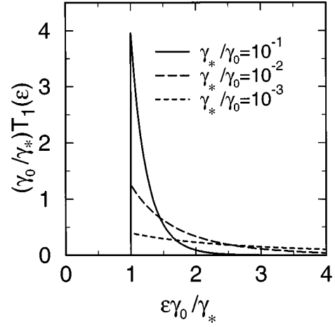
FIG. 2. Probability distribution of the lasing threshold in a cavity with small absorption in the boundary and a single hole ( \nu = 1 ), computed as -dp_1(\varepsilon)/d\varepsilon from Eq. (14). We chose \Omega/\delta\omega_0 = 10 and took three values of \gamma_*/\gamma_0 such that \gamma_*/\gamma_0 is much smaller than, equal to, or much greater than (\delta\omega_0/\Omega)^{2/\nu} = 10^{-2} .
