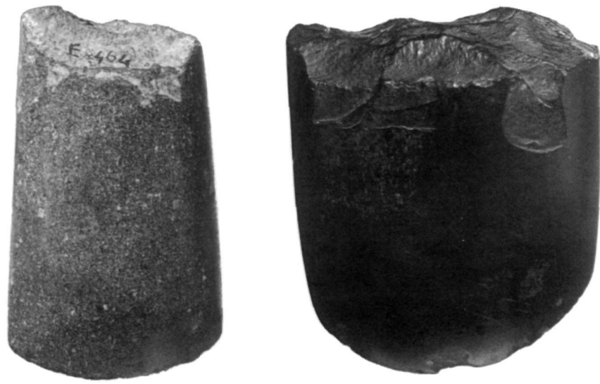
Fig. 21 Adzes obviously rehafted after having been broken. Left: Elsloo 464, found in a grave. Right: Elsloo 19 with a lustre on the fracture, thought to have resulted from rehafting. 1:1.
