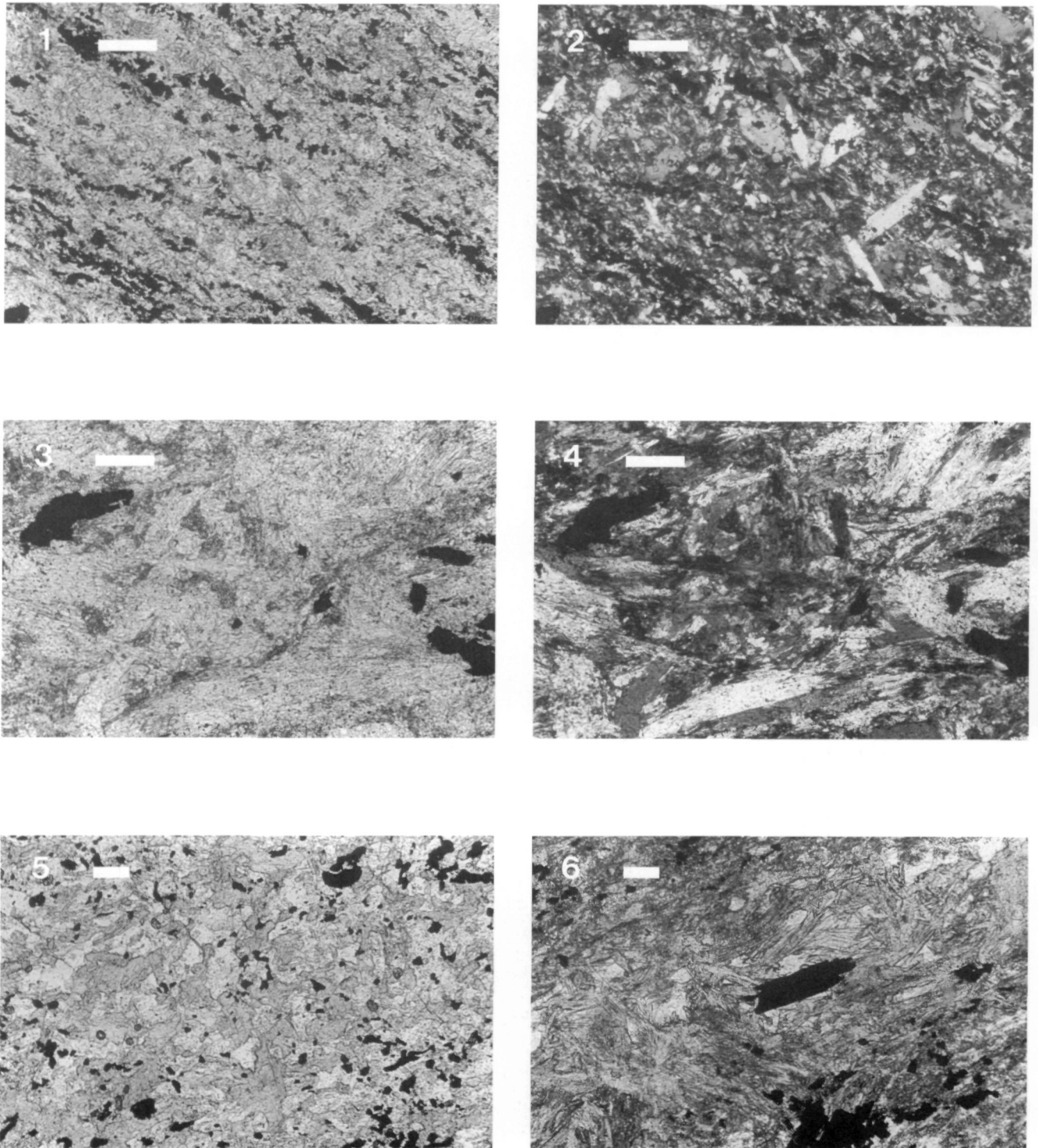
Fig. 12 Examples of amphibolite, thin sections, scale unit 100 \mu m. 1. Langweiler 9, 146-339, banded amphibolite rich in opaque minerals; the actinolitic hornblende crystals are partly arranged in sheaves 2. as 1. crossed nicols 3. Langweiler 9, 1010-8, hornblende in sheaf-like clusters 4. as 3, crossed nicols 5. Vlijtingen K49.16-78, amphibolite with well-crystallized bluish-green hornblende 6. Langweiler 8, 3078-5, amphibolite with typical sheaves of actinolitic hornblende crystals.
