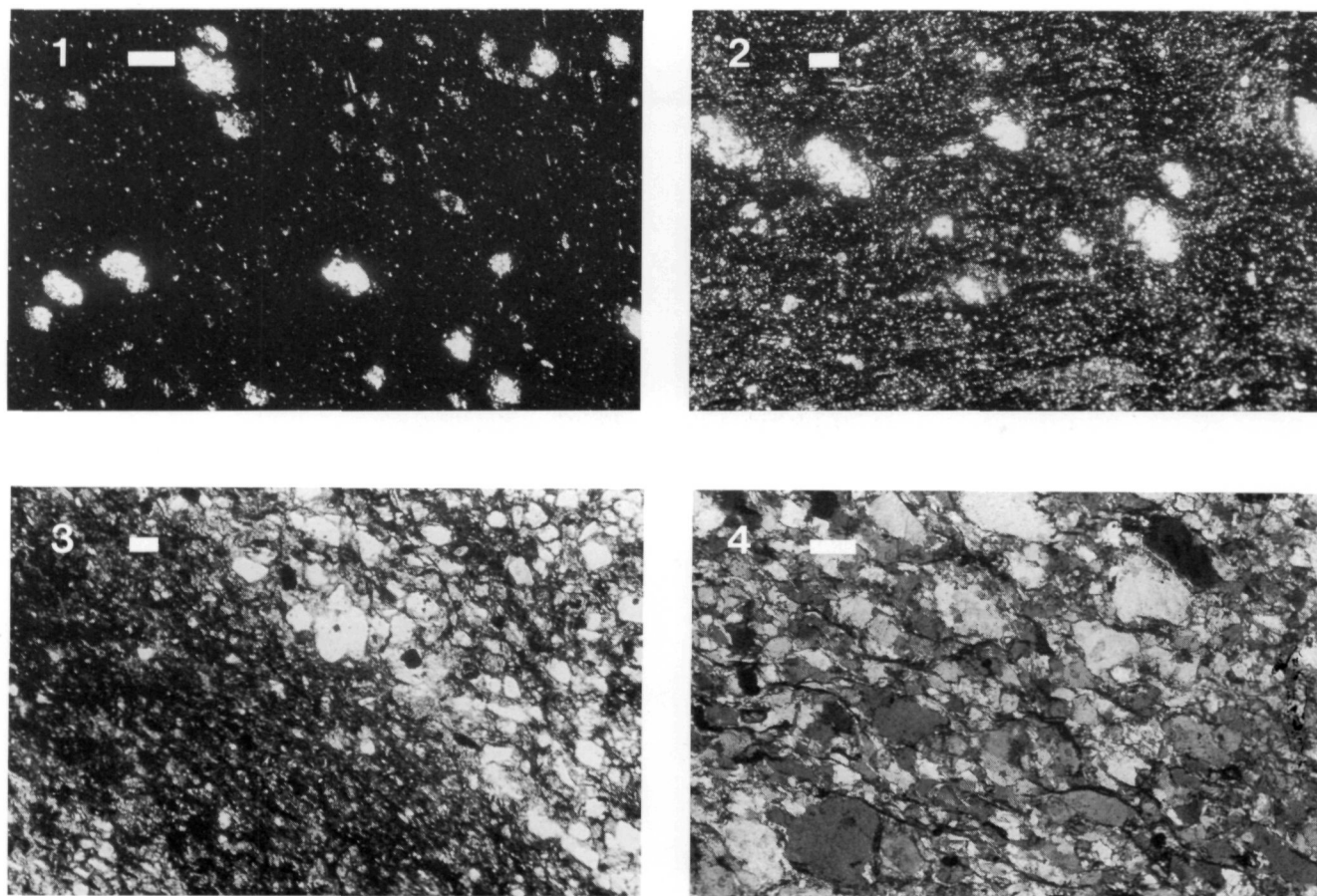
Fig. 14 Examples of siliciclastic rocks, thin sections, scale unit 100µm. 1. Aubechies Coron-Maton F 4, lydite 2. Wange, lydite, richer in crypto-crystalline quartz 3. Blicquy Petite Rosière 17-386 grès de Horion-Hozémont 4. Langweiler 8, 1702-6 weakly deformed quartzite.
