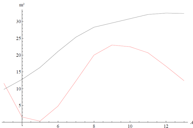
Figure 3.4. The values of the masses of the first two excitations of the tachyon as a function of the parameter A of the tachyon potential (3.119). The m_1^2 (rescaled by a factor of ten) is plotted in red and the m_2^2 is plotted in black.
