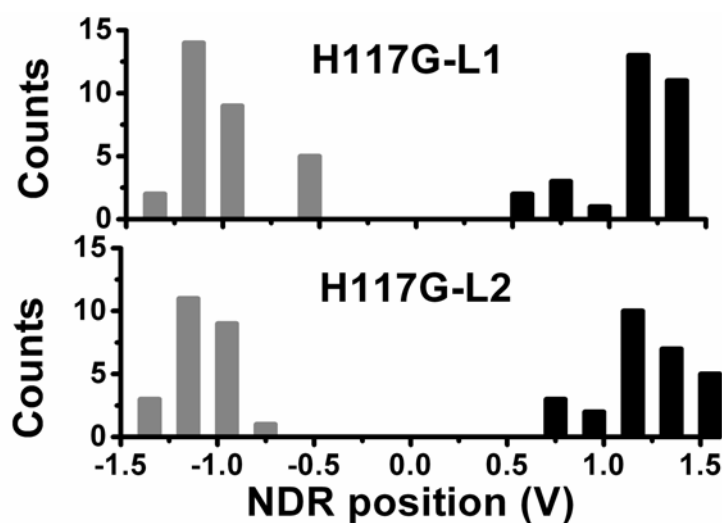
Figure 11. Histograms presenting the variation of NDR peak locations (V) for H117G-Cu reconstituted with either linker.
