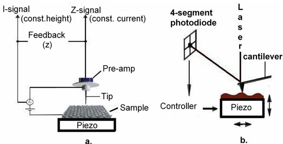
Figure 3. Architecture of the scanning tunneling microscope (a) and of an atomic force microscope (b)
