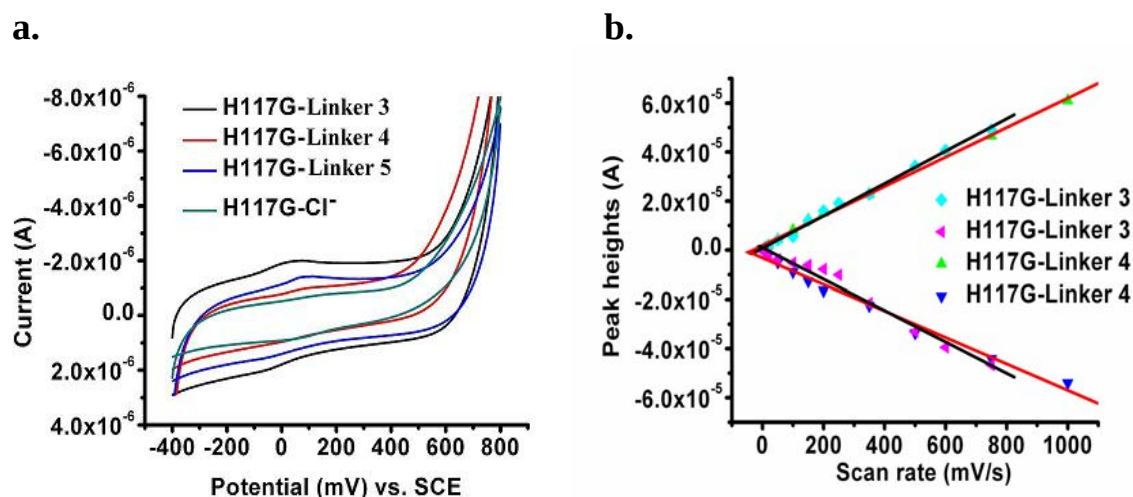
Figure 4. a) Cyclic voltammograms of 100 \mu\text{M} H117G-Cu reconstituted with linkers \text{L}_3 , \text{L}_4 , \text{L}_5 and \text{Cl}^- and assembled on PGE electrodes; scan rate for all scans is 10mV/s; measurements performed in 150mM \text{Na}_2\text{SO}_4 and 20mM MES pH 6.0, at room temperature b) Examples of the scan rate dependence of azurin H117G-Cu reconstituted with linkers 3 and 4, demonstrating the adsorbed nature of the complexes.
