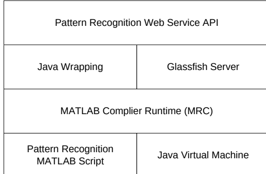
Figure 6-13 underline structure of the pattern recognition API
