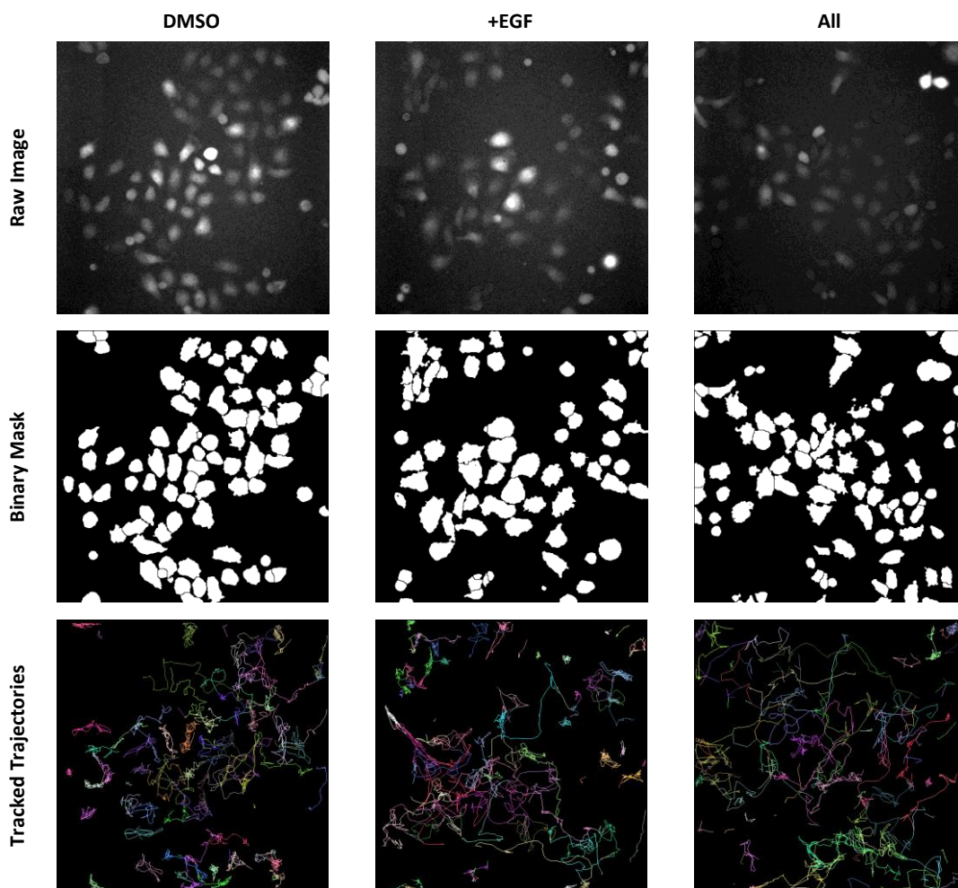
Figure 4-2 segmentation and tracking results for the different GF treatments
