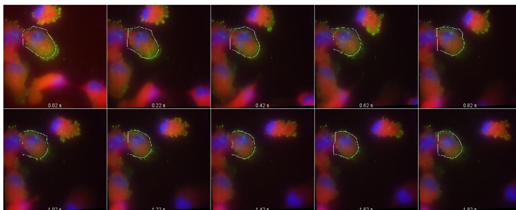
Figure 5-12 montage of low-motile cell
