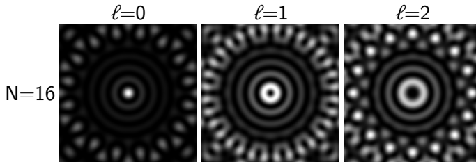
Figure 3.4: Far-field intensity patterns behind an multipoint interferometer of N = 16 points illuminated by a Laguerre-Gaussian beam with vorticity \ell . The intensity patterns hint at the fact that the patterns converge to a Bessel function in the limit that N \rightarrow \infty as described by equation 3.3.
