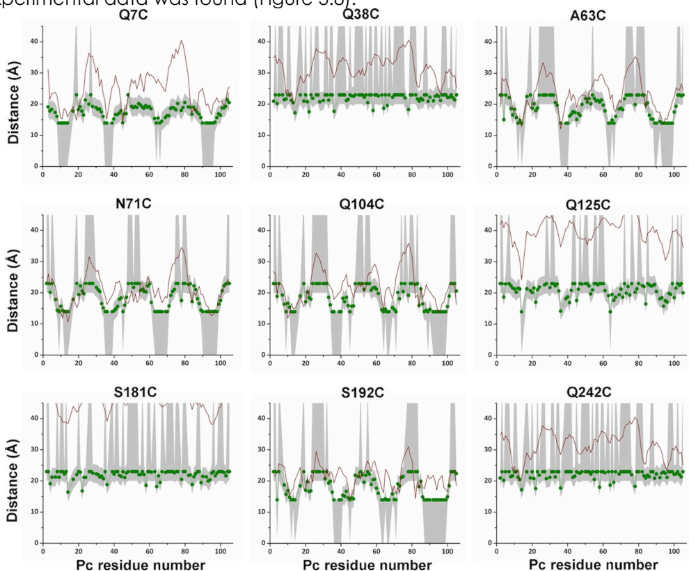
Figure 3.8. Comparison between back calculated averaged distances from 2000 randomly selected structures of the MC simulation (red line) assuming f_1 = 1 and the experimental distances (green circles and lines). The grey areas indicate the error margins of experimental data.
