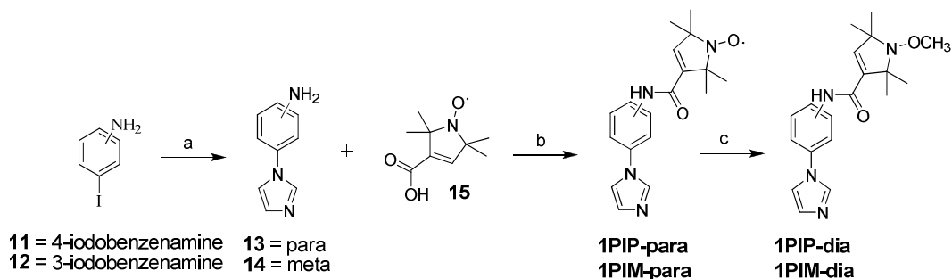
Scheme 3. Synthesis of spin labeled 1-phenylimidazole analogs. (a) imidazole, CuI, K 3 PO 4 , DMF, 40 °C 40 h; (b) HATU, TEA, DMF, RT, 12 h; (c) FeSO 4 ·7H 2 O, H 2 O 2 , DMSO.
