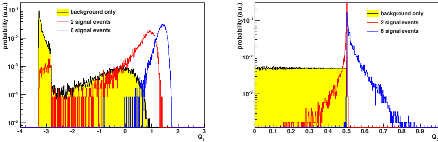
Figure 7.8.: Distribution of the variables Q_1 (left) and Q_2 (right) for background only experiments (yellow histogram) and for the cases where we simulate two (red histogram) and six signal events (blue histogram) at a declination \delta = -70^\circ .
