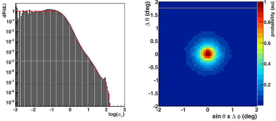
Figure 7.3.: Left: Distribution of the point spread function as a function of the reconstruction angle, \alpha_{rec} , for simulated E^{-2} neutrinos. The red line shows the parametrisation used in the likelihood fit. Right: PSF in terms of \delta\theta , the difference in the zenith angle between the true neutrino direction and the reconstructed muon direction, and the angular distance on the azimuth direction. In both plots all the final cuts of the analysis are applied.
