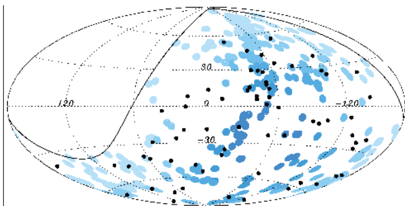
Figure 1.2.: Sky map in galactic coordinates of the 69 arrival directions of CRs with energy E \geq 55 EeV detected by the PAO up to December 2009 (black dots). Blue circles of radius 3.1^\circ show the locations of the 318 selected AGNs within 75 Mpc. The darker is the blue the larger is the relative exposure. The solid line represents the field of view of the PAO for zenith angles smaller than 60^\circ . The figure is taken from [10].
