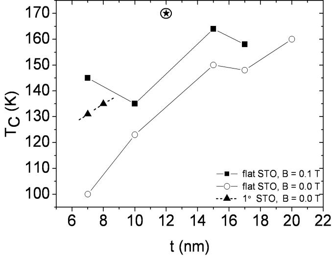
Figure 4.6 — The Curie temperature as function of film thickness. Determined from M vs T at B = 0 T (circles) and B = 0.1 T (squares). The triangles show T_C for two films grown on 1° STO and the star shows T_C for sample L(10). The drawn and dashed lines are guides to the eye.
