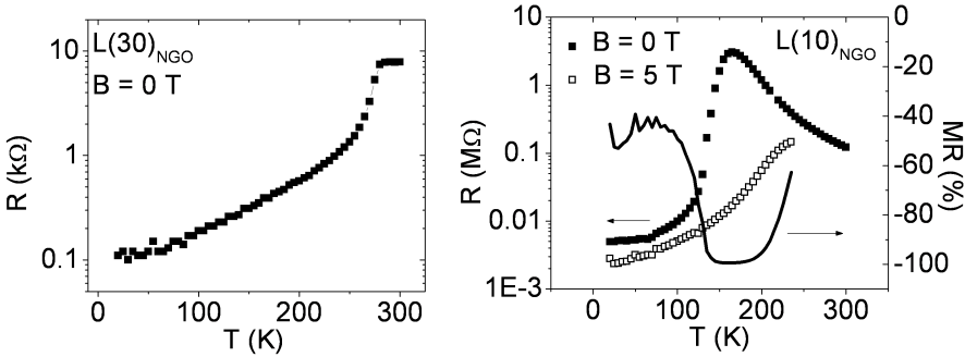
Figure 5.8 — a) R(T) behavior of microbridge L(30) NGO ( J = 7 \times 10^5 \text{ A/m}^2 , 0.1 \mu\text{A} ). b) R(T) behavior of microbridge L(10) NGO ( J = 2 \times 10^6 \text{ A/m}^2 , 0.1 \mu\text{A} ) measured in both B = 0 \text{ T} and B = 5 \text{ T} . The calculated magnetoresistance as function of temperature is also shown (solid line). Both microbridges have a width of 5 \mu\text{m} .
