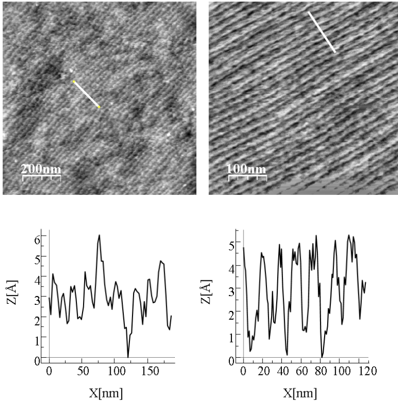
Figure 3.2 — AFM images of STO substrates and corresponding profiles of (left) untreated STO (scale bar: 200 nm) and (right) \text{TiO}_2 terminated STO (scale bar: 100 nm); both substrates have a misorientation of 1^\circ towards the [010] direction.
