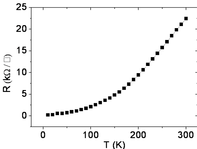
Figure 3.15 — Sheet resistance vs. temperature of the 30 sec Ar-etched STO sample ( 1.5 \times 2.6 \text{ mm}^2 ) obtained from I-V curves at I = 20 \text{ } \mu\text{A} .
