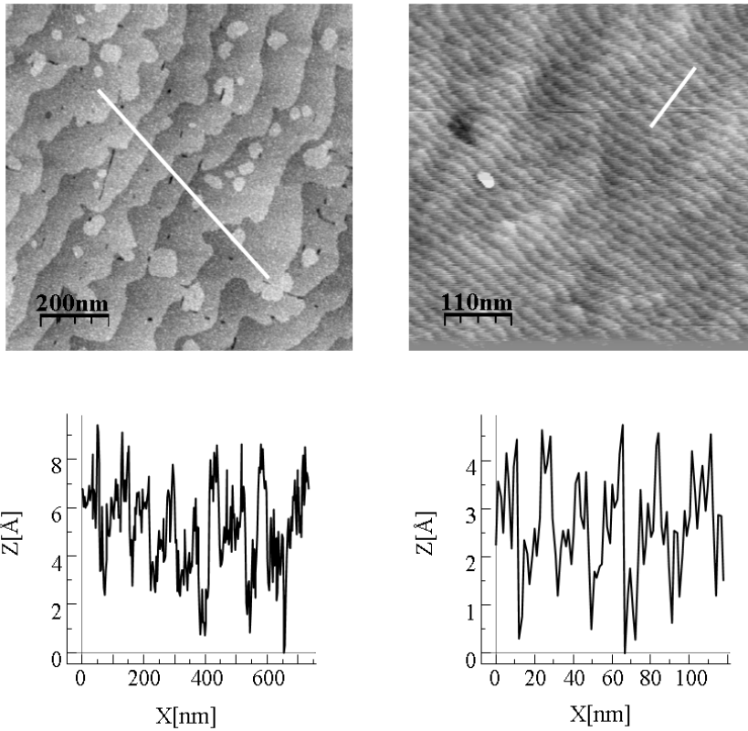
Figure 3.3 — AFM images of LCMO thin films and corresponding profiles of (left) 15 nm LCMO on flat STO, L(15) (scale bar: 200 nm) and (right) 7 nm of LCMO on untreated STO with a misorientation of 1^\circ , L(7) mis (scale bar: 110 nm).
