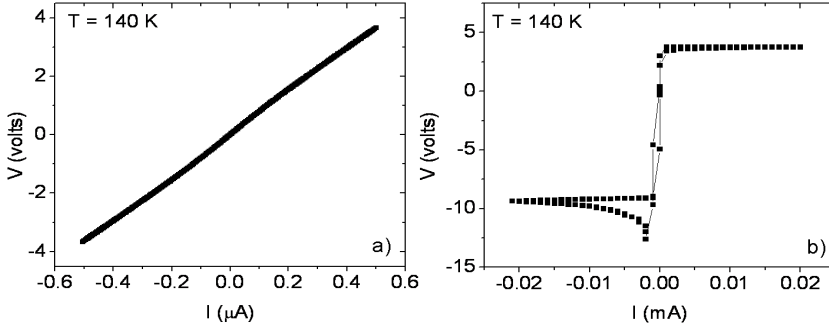
Figure 3.16 — a) I-V curve of 30 sec Ar-etched STO ( 1.5 \times 2.6 mm 2 ) at T = 140 K before and b) after 2 min of oxygen plasma treatment. The high resistance between the current contacts leads to saturation of the current source.
