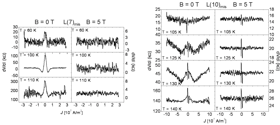
Figure 5.11 — a) Numerical derivatives of the measured I-V curves for 1 \mu\text{m} wide microbridge L(7)_{\text{mis}} . b) Numerical derivatives of the measured I-V curves for the 5 \mu\text{m} wide microbridge L(10)_{\text{mis}} . For all curves the temperature and the magnetic field at which the curve was measured is indicated.
