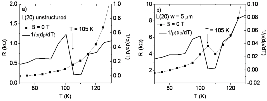
Figure 6.2 — R(T) behavior of sample L(20) a) unstructured and b) microbridge ( w = 5\ \mu\text{m} ) between T = 70 - 130 K. Right axis: 1/\rho(d\rho/dT) (solid line). The position of the phase transition in the STO is indicated by the arrow. Similar behavior is observed in ref. [9].
