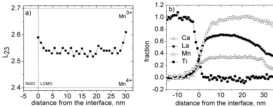
Figure 3.11 — a) The L_{23} ratio across the L(30) NGO . b) Elemental composition of the same sample.
