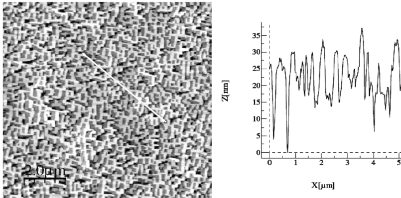
Figure 3.1 — (Left) AFM image (scan size: 10 \times 10 \mu\text{m}^2 ) and (right) profile of 75 nm LCMO film on a STO substrate as an example of morphology due to slow growth rate. Scale bar: 2 \mu\text{m} .
