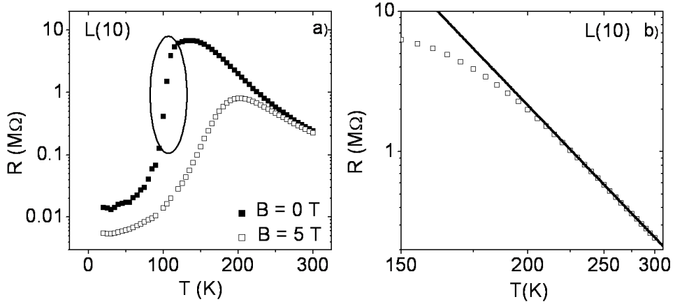
Figure 5.1 — a) Typical R(T) behavior with CMR effect for the 5\ \mu\text{m} wide microbridge L(10) with J = 1 \times 10^7\ \text{A/m}^2 . We observe nonlinear I-V curves in the range which is indicated by the ellipse. b) Log R vs. T plot for high temperatures T = 150 - 300\ \text{K} . Note: the scale on the T -axis is reciprocal in order to it to 1/T -behavior. The solid line is a fit to the data to extract the activation energy, E_A = 112\ \text{meV} for the thermally activated polaron hopping process.
