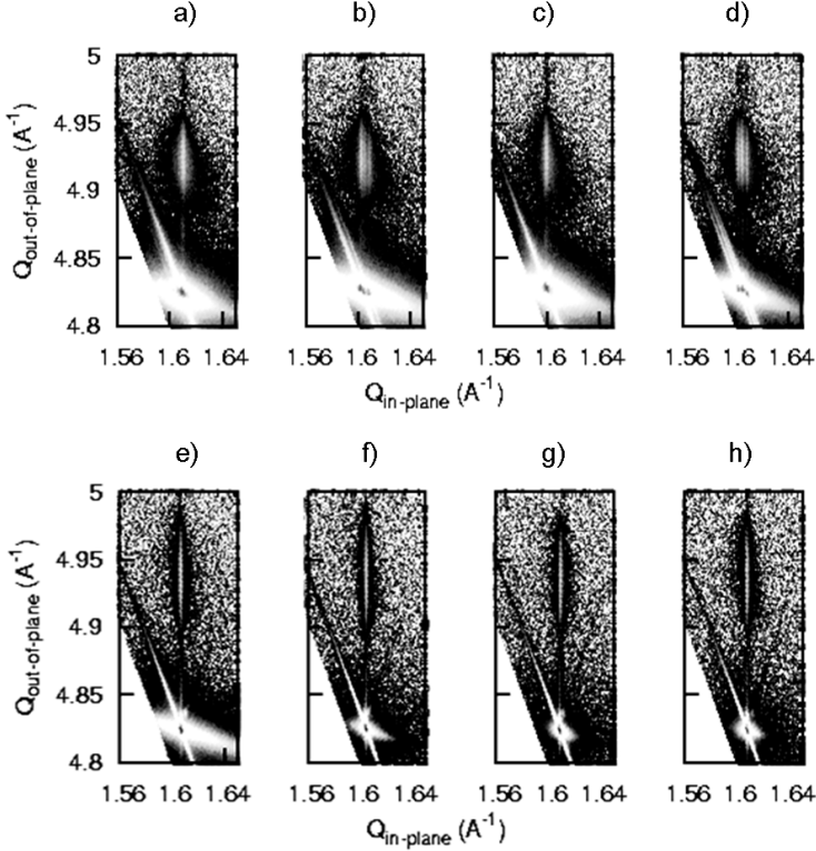
Figure 3.5 — The RSM-plots of two samples are shown for reflections (103) (a and e), (013) (d and f), ( \bar{1}03 ) (c and g) and ( 0\bar{1}3 ) (b and h). Graphs a-d): L(20), graphs e-h): L(10). For each graph two peaks are visible, the strong peak at the bottom (at 1.6 \text{ \AA}^{-1} and 4.82 \text{ \AA}^{-1} ) is caused by the STO substrate and the weaker peak at the top (around 1.6 \text{ \AA}^{-1} and 4.94 \text{ \AA}^{-1} ) is caused by the LCMO film.
