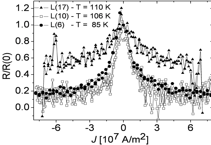
Figure 5.5 — Numerical derivatives dV/dI of the nonlinear I-V curves for three different microbridges on STO. Note: the curves are normalized w.r.t. the zero bias resistivity. For each curve the sample name is indicated as well as the temperature at which the I-V curve was measured. For all films the curves are shown for the temperature where the largest reduction as function of applied current occurred. The zero bias resistances are, L(17): R(0) = 0.3 \text{ M}\Omega , L(10): R(0) = 4.0 \text{ M}\Omega and L(6): R(0) = 4.3 \text{ M}\Omega .
