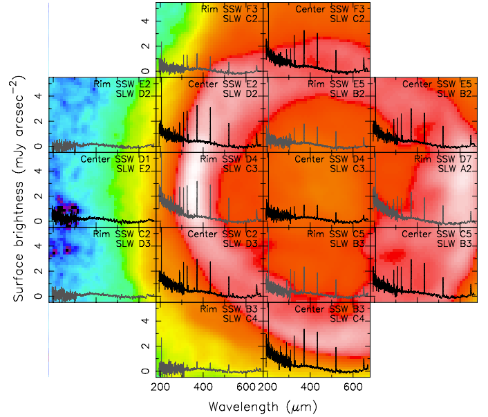
Fig. 9. Spectra of NGC 6781 over the complete SPIRE spectral coverage (194–672 μm) at 16 distinct positions, where the SSW and SLW bolometers spatially overlap reasonably well. Bolometer positions are nested between the two pointings, and spectra extracted from the center pointing are shown in black and those from the rim pointing are shown in dark gray. The background PACS 70 μm image indicates the approximate locations of the corresponding bolometers within the nebula. The flux units are set to the surface brightness (mJy arcsec -2 ). The measurements are valid roughly within the central 30'' of the specific location of the bolometers. The spatial variation of the strength of the CO rotational transition lines and thermal dust continuum is clearly detected.
