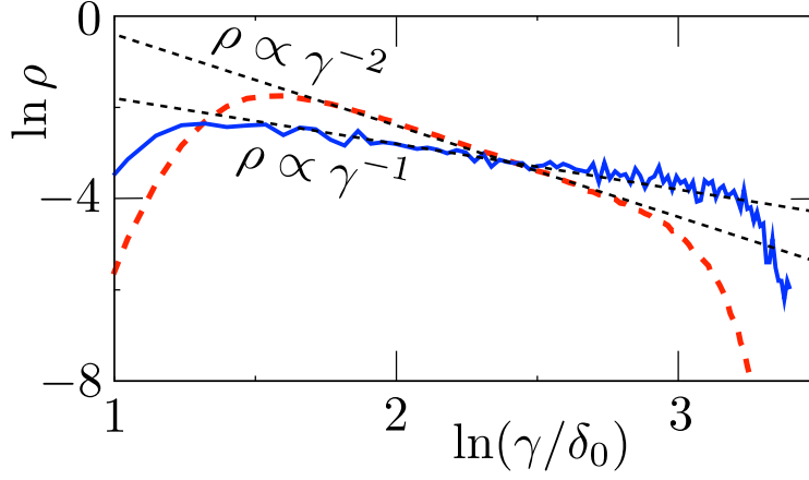
Figure 5.4. Double-logarithmic plot of the probability distribution \rho(\gamma) , normalized to unity, of the imaginary part \gamma of the poles of the scattering matrix. The curves are calculated by averaging over some 2000 realizations of the class-D ensemble, with N = 10 , M = 500 , \Gamma = 0.9 . The red dashed curve includes all poles, while the blue solid curve includes only the poles on the imaginary axis ( E = 0 ). The black dashed lines are the predicted slopes from Eq. (5.16) and (5.20).
