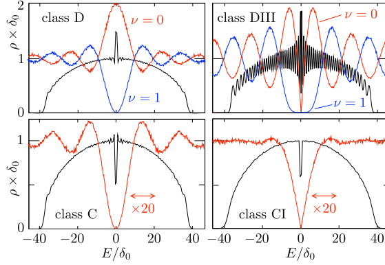
Figure 5.8. Black and red curves: Average density of states in the four Altland-Zirnbauer ensembles, calculated numerically for Hamiltonians of dimension M \times M = 60 \times 60 in classes C, CI, D, and M \times M = 120 \times 120 in class DIII (when each level has a twofold Kramers degeneracy; \rho and \delta_0 refer to distinct levels). The black curve shows the full semicircle, the red curve shows the region around E = 0 (horizontally enlarged by a factor 20). These are all results for a topologically trivial superconductor, without a zero-mode ( \nu = 0 ). The blue curves (labeled \nu = 1 ) show the effect of a zero-mode in class D ( M = 61 ) and class DIII ( M = 122 ). The delta-function peak from the zero-mode itself is not plotted.
