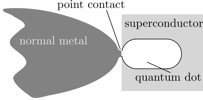
Figure 5.2. Schematic illustration of an Andreev billiard.
