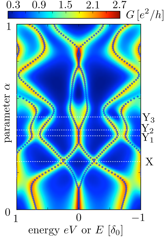
Figure 5.6. Parametric evolution of the differential conductance G(V, \alpha) (color scale) and the real part E of the poles of the scattering matrix S_\alpha(\varepsilon) . These are results for a single realization of the class D ensemble with M = 120 , N = 6 , and \Gamma = 0.3 .
