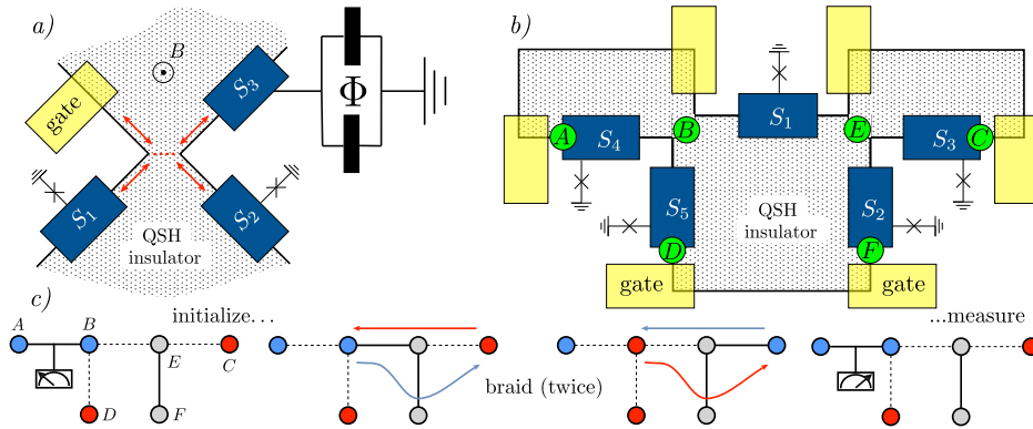
Figure 3.4. a) Constriction in a quantum spin-Hall insulator, contacted along three edges by a superconducting island. If the fourth edge is blocked by a gate electrode, the constriction traps a Majorana fermion. Each superconducting island is connected to a superconducting ground by a split Josephson junction enclosing a magnetic flux, indicated schematically by a \times symbol and shown expanded for one of the islands. b) Two constrictions in series form a \pi -shaped circuit that can be used to braid the Majorana fermions (green circles). The flux through each split Josephson junction controls the coupling of adjacent Majoranas. c) Schematic of the braiding operation in the \pi -circuit [38]. Coupled Majoranas are connected by a solid line, uncoupled Majoranas by a dashed line.
