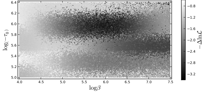
(a) WiggleZ
