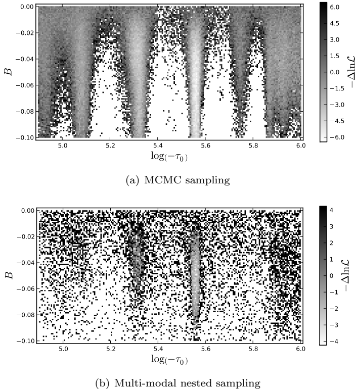
Figure 3.2: Profile likelihood in the (\ln(-\tau_0), B) plane for Planck+WiggleZ, for the different sampling methods. It demonstrates how the multi-modal nested sampling algorithm samples more thoroughly the regions of low likelihood. The regions not samples are shown in white (in the B&W version, not to be confused with the light grey areas of high likelihood). The difference in the likelihood ( \Delta ) is calculated against the best fit value of \Lambda CDM in the different data sets.
