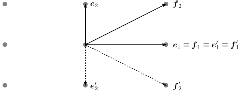
Figure 5.3: Two different bases for the p-rectangular lattice: \mathfrak{e} = \{e_1, e_2\} and \mathfrak{f} = \{f_1, f_2\} , and the action of the point group generator (primed vectors).
