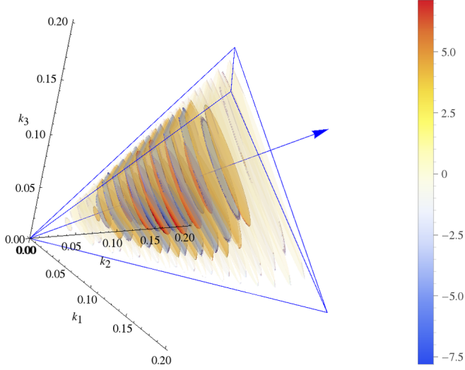
(a) Full 3D primordial bispectrum (in colour in the on-line version of [1])
