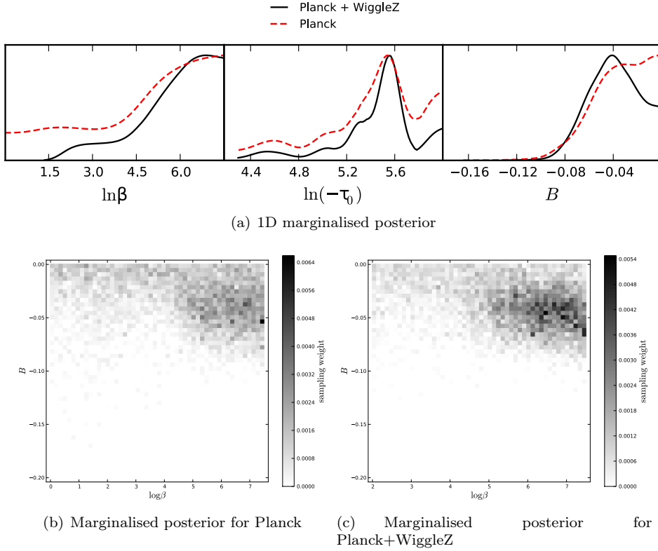
Figure 3.3: Multi-modal nested sampling results: 1D marginalised posterior distribution for the feature parameters and 2D marginalised posterior distribution in the plane (\ln \beta, B) , with and without the WiggleZ data set. Notice how the addition of the WiggleZ data set increases the overall likelihood of a feature with a non-zero amplitude.
