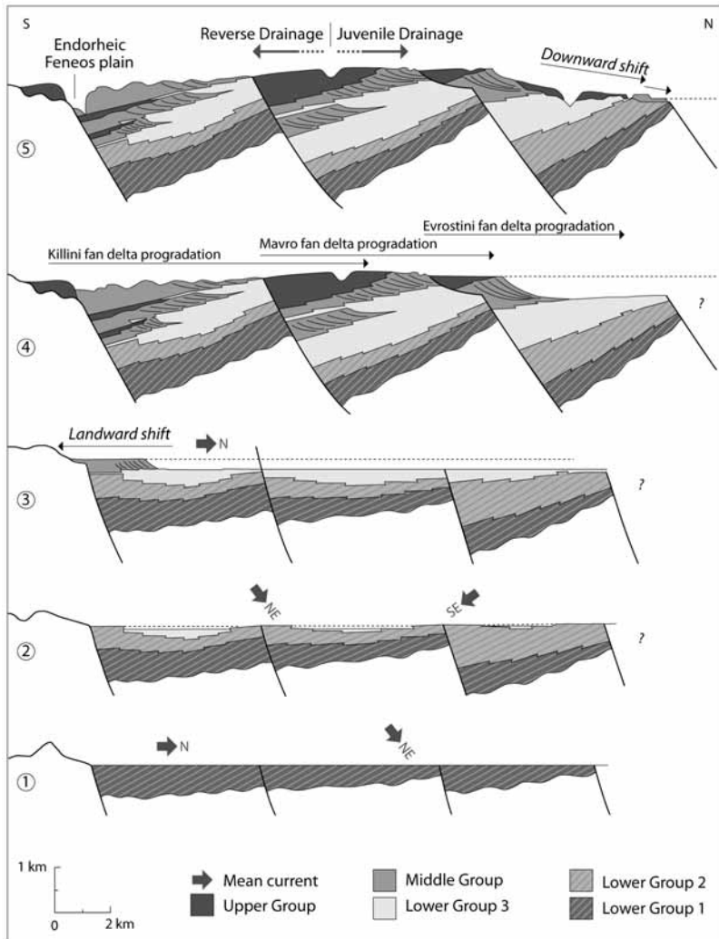
Fig. 6.15 Palaeogeographic and tectono-sedimentary evolution of the Akrata-Derveni area. Vertical exaggeration \times 4 . Modified after Rohais et al. 2007: fig. 10
