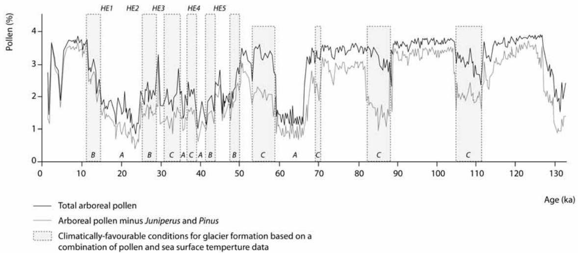
Fig. 6.6 Last glacial pollen curves from Ioannina (I-284) and potential intervals favoring glacial formation. A: major stadials characterized by low arboreal pollen; B: intermediate periods between the peaks of stadials/interstadials; C: intervals characterized by large differences between total arboreal pollen frequencies and arboreal pollen frequencies excluding Pinus and Juniperus . Heinrich events (HE) are also shown. Modified after Hughes et al. 2006a: fig. 5
