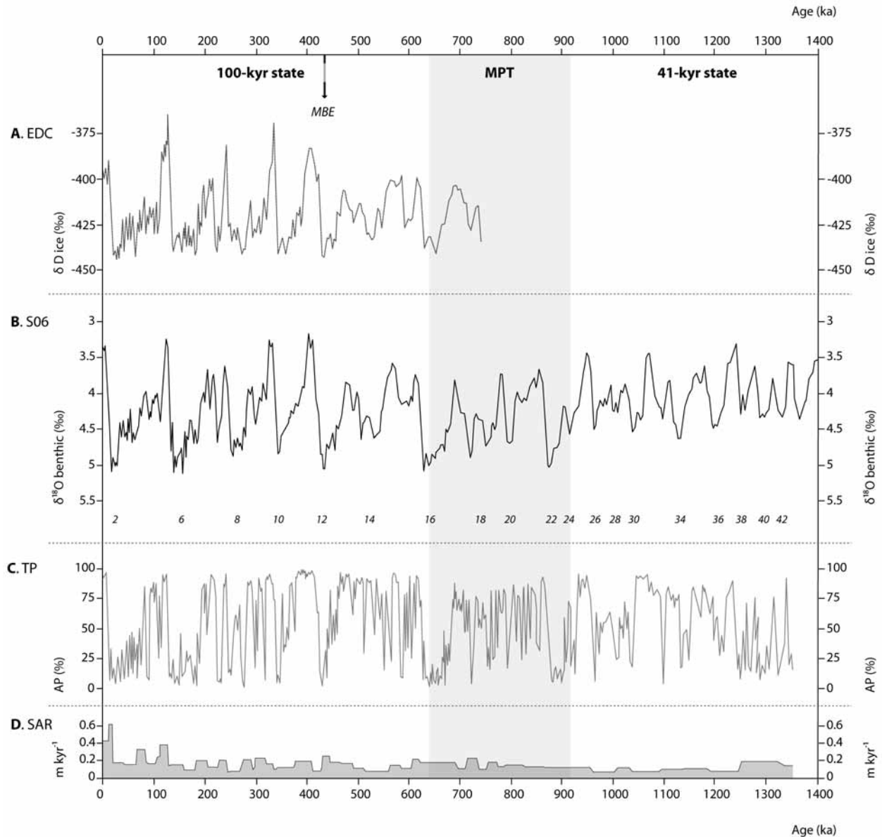
Fig. 6.3 The Tenaghi Philippon Arboreal Pollen (AP) curve (C) plotted on the pollen-orbital derived timescale and compared to (B) the S06 \delta^{18}O benthic composite record from sites in the equatorial East Pacific and (A) the EPICA Dome C Deuterium ( \delta D ) record from Antarctica. Glacial marine isotopic stages, sediment accumulation rates (D), the mid-Pleistocene transition (MPT) and the position of the mid-Brunhes event (MBE) are also indicated. Modified after Tzedakis et al. 2006: fig. 5
