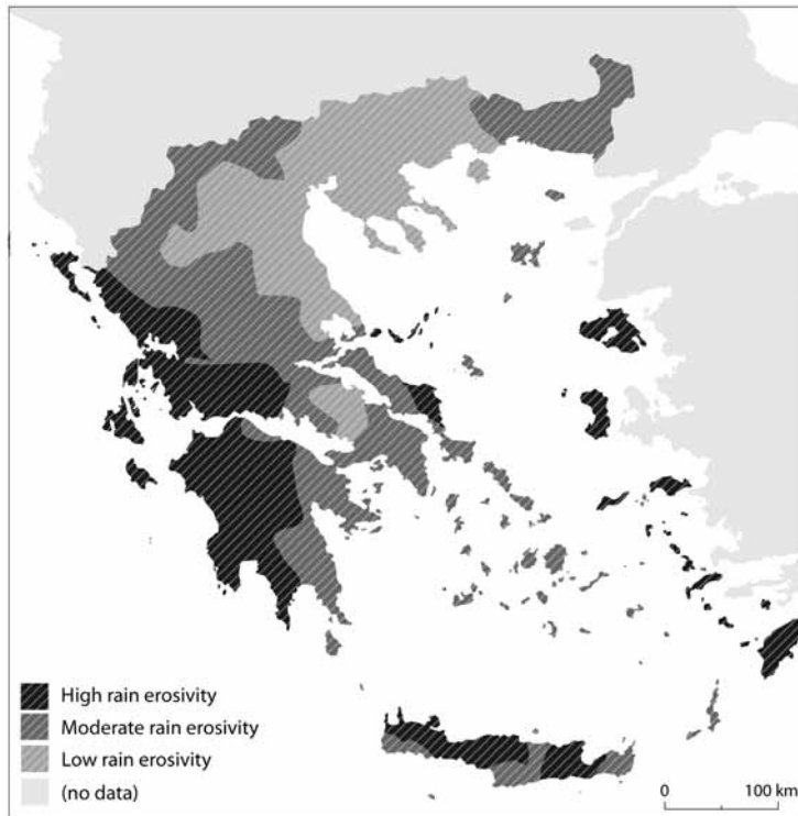
Fig. 6.2 Rain erosivity map of Greece, modified after Kosmas et al. 1998b: fig. 15.2. Areas of 'high rain erosivity' experience rainfalls that are unevenly distributed throughout the year; they commonly come in the form of intense storms of short duration and occur during dry seasons
