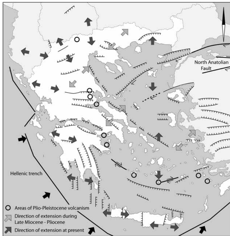
Fig. 6.10 Extensional tectonism and major faults in the Aegean region. Black arrows show the movement of the African plate and the direction of compression in the Ionian Sea. Modified after Mountrakis, university notes
