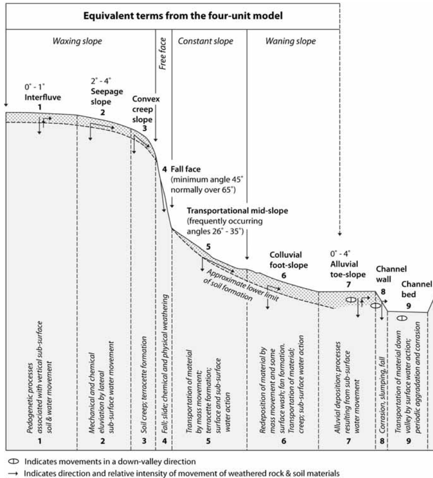
Fig. 6.27 The nine-unit land-surface model of Delrymple et al. (1968). Modified after Clark and Small 1982: fig. 5.10
