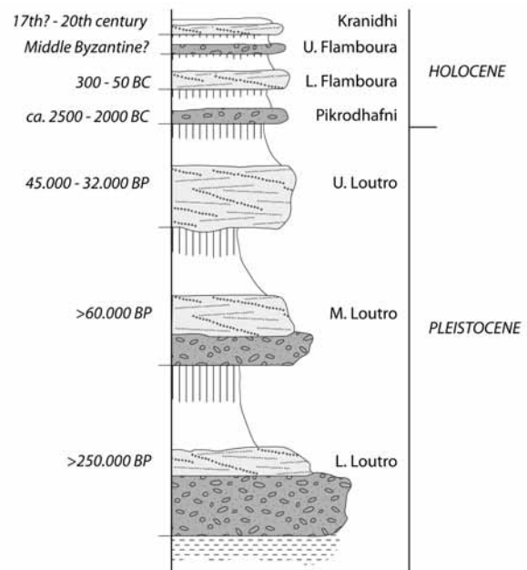
Fig. 6.23 Quaternary alluvial sequence from southern Argolid (Peloponnese). Cobbles with a chaotic structure indicate debris flows, whilst stratified gravels are streamflood deposits; blank zones are overbank loams and vertical lines denote soil profiles. Although the dates give only approximate ages, they do highlight an apparent discontinuity in alluviation events. Modified after van Andel et al. 1986: fig. 4
