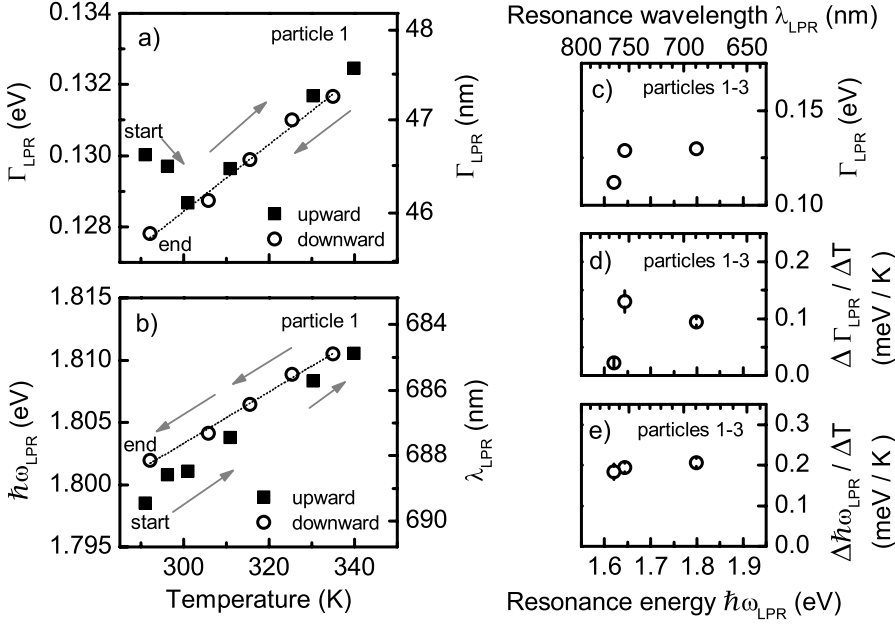
Figure 5.3: Temperature dependence of the longitudinal plasmon resonance of single gold nanorods, immobilized on a glass substrate and surrounded by immersion oil. (a) Width \Gamma_{\text{LPR}} and (b) energy \hbar\omega_{\text{LPR}} of the longitudinal plasmon resonance of an individual gold nanorod. Data was taken first going upwards in temperature, then downwards back to room temperature at 290 K. The dotted lines are linear fits of the data from the series downwards in temperature. (c-e) Measured temperature dependence of the plasmon for the nanorod in (a-b), plus two additional rods, as a function of the longitudinal plasmon resonance energy \hbar\omega_{\text{LPR}} of the rods. Panel c): Width \Gamma_{\text{LPR}} (at 290 K) of the rods. Panels (d) and (e) display respectively the temperature dependence of the plasmon width and energy, obtained from the slopes of the linear fits as in (a-b).
